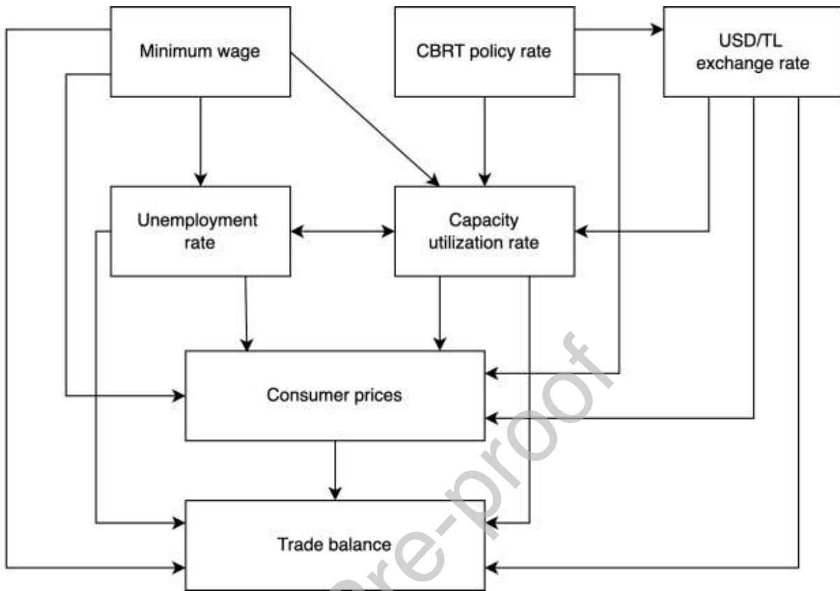
Fig. 4. The contemporaneous effects in the Structural Vector Autoregression (SVAR) specification (Models 8 and 9).
