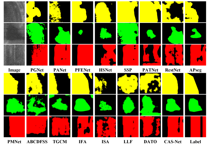
Fig. 10. Visual comparison of segmentation performance on the Agriculture-Vision dataset.
