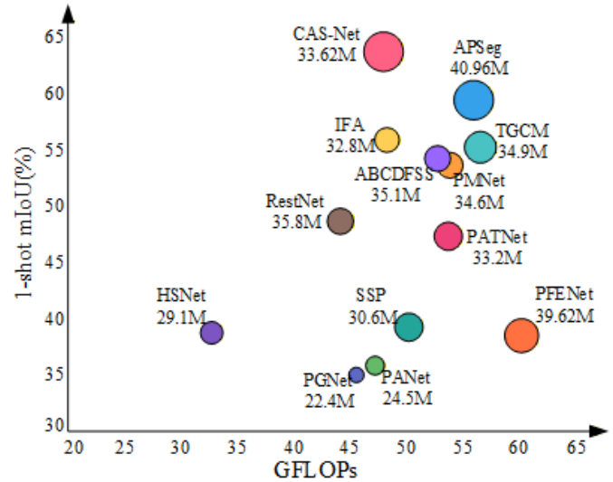
Fig. 8. Comparison of computational efficiency and model size among different methods. The horizontal axis represents computational cost (GFLOPs), and the size of each circle corresponds to the number of parameters (Params). Different colors indicate different methods.
