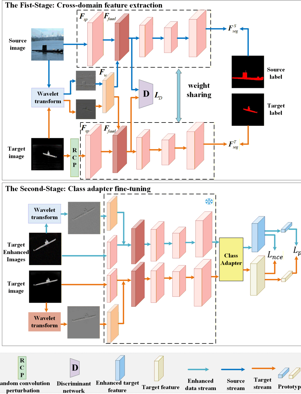
Fig. 2. Overview of the proposed two-stage Cross-Domain Few-Shot Semantic Segmentation framework.
