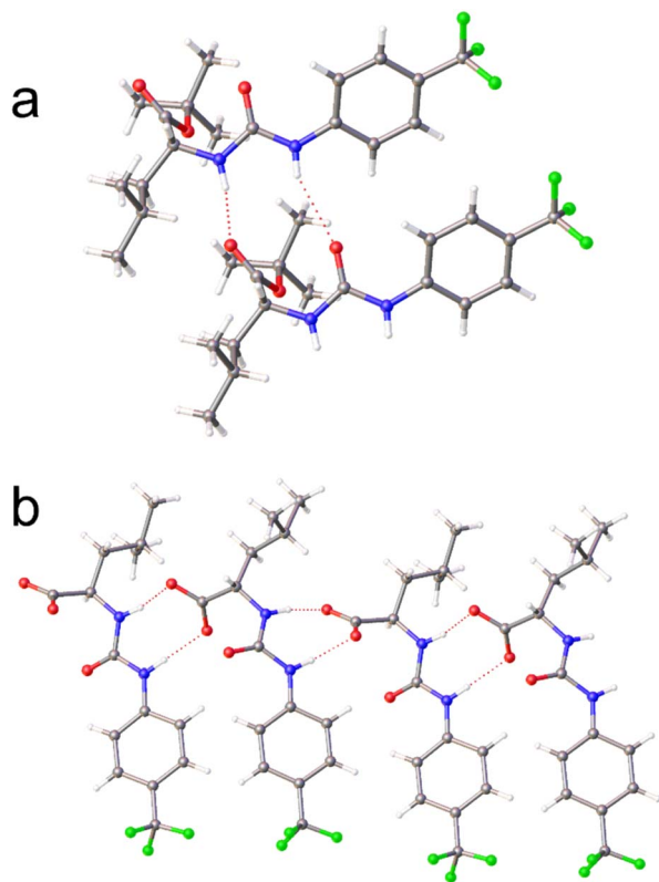
Fig. 2 Single crystal X-ray structure of (a) 2 and (b) the 1:1 enantiomeric mixture of 3 and 5 . The TBA counter cations have been omitted for clarity. Grey = carbon, blue = nitrogen, red = oxygen green = fluorine, white = hydrogen, red dashed lines = hydrogen bonds. †1
