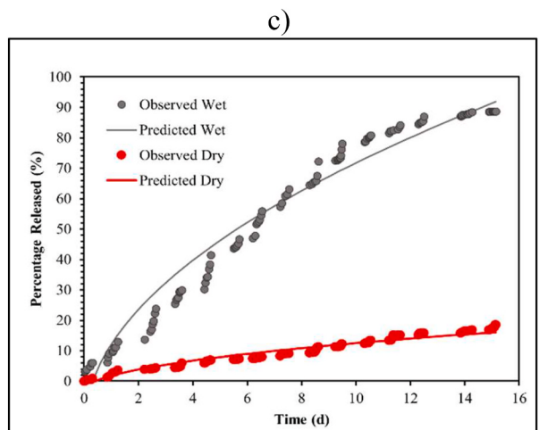
c) Higuchi Model
