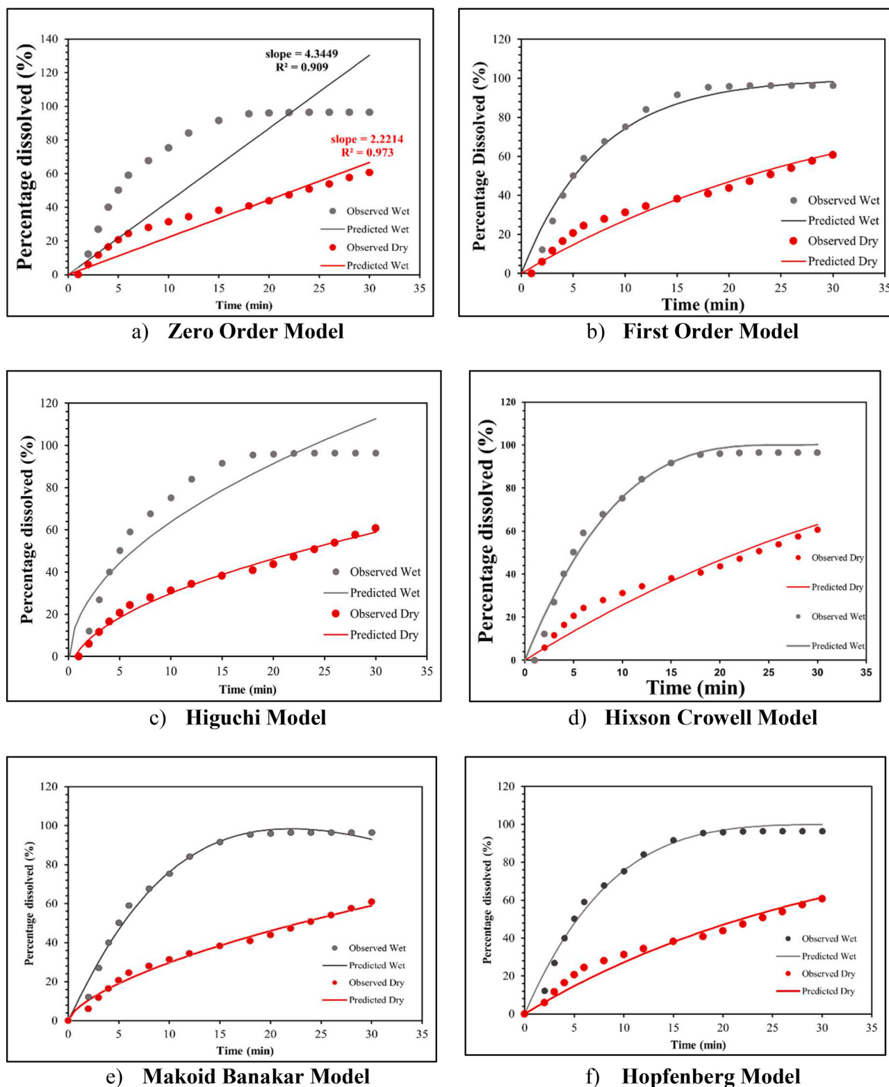
Fig. 5. Kinetic Release Models for fibres submerged directly in PBS.
