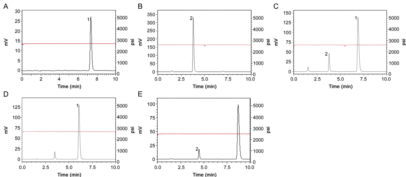
Fig. 5. Typical HPLC chromatograms of DIL standard solution at 25 °C (A) and DIL recovered from MAS-DIL complex using 2 M HCl (24 h exposure) (B), 2 M HCl (30 min exposure) (C), ultra – pure water (D) and pH 6.8 phosphate buffer (E) showing the presence of DIL (1) and degradant desacetyl diltiazem (2).
