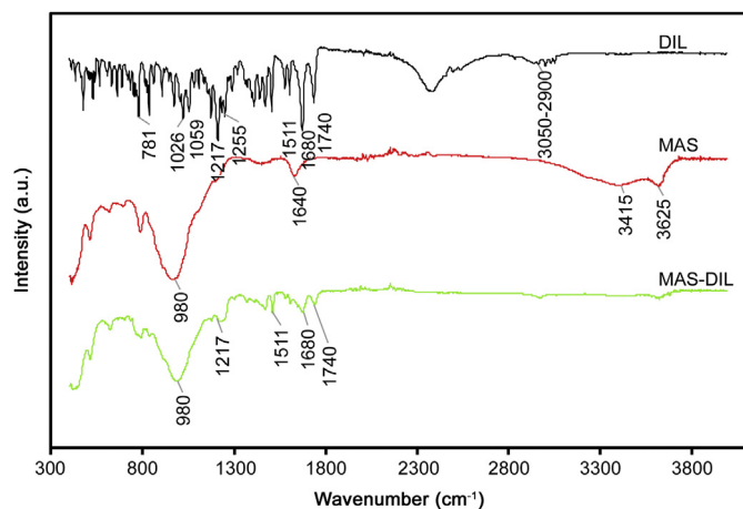
Fig. 6. ATR-FTIR for DIL, MAS and MAS-DIL double drug loaded complex.
