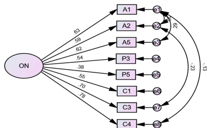
Fig. 2. CFA 1-factor structure goodness-of-fit model.
