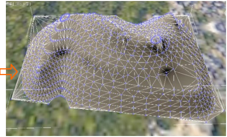
(f) Generation of a 3D terrain geometry by assigning triangle primitives to triangulation patches. Automatic texture mapping onto triangles
