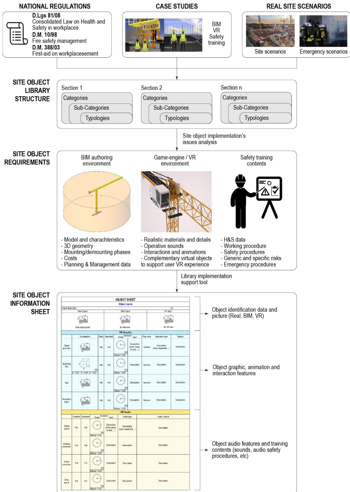
Fig. 2: Site Object Library development workflow
