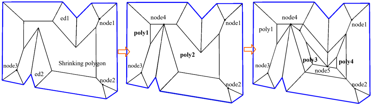
(a) Shrinking polygon just before a split event. Edge events give rise to \text{node1} \sim \text{node3}
