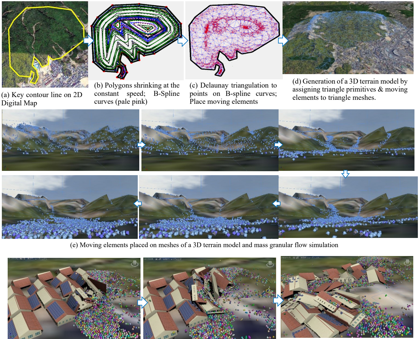
(a) Key contour line on 2D Digital Map (b) Polygons shrinking at the constant speed; B-Spline curves (pale pink) (c) Delaunay triangulation to points on B-spline curves; Place moving elements (d) Generation of a 3D terrain model by assigning triangle primitives & moving elements to triangle meshes. (e) Moving elements placed on meshes of a 3D terrain model and mass granular flow simulation (f) Interaction between mass moving elements and 3D building model made up of parts for dynamic simulation Fig.8: Automatic generation process of a 3D terrain model by straight skeleton computation and mass granular flow simulation, collapse of 3D building models hit by a debris flow
