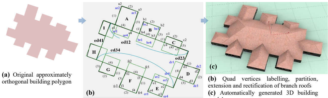
Fig.6: Partition, extension and rectification of branch roofs by quad vertices labelling
