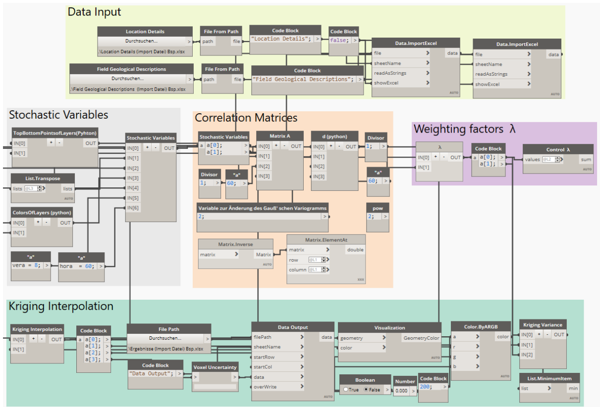
Fig. 2: Dynamo script
