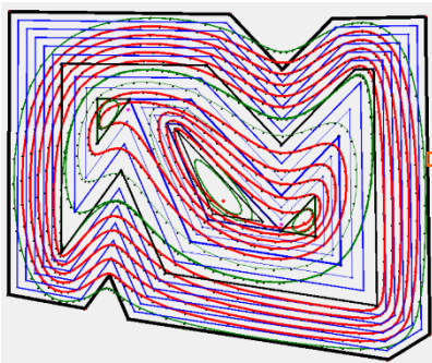
(d) Polygons shrinking at the constant speed; Polygons (blue) at Split event. B-Spline curves (red) from these polygons
