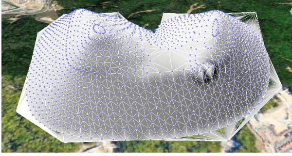
Fig.4: Generation of a 3D terrain geometry by assigning triangle primitives to triangulation patches
