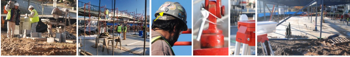
Fig. 2: Images of work environment (concrete masonry unit saw and columns), UWB tag on worker's helmet and UWB tags on mobile crane hook, UWB reference tag on tripod and UWB receiver (from left to right image)
