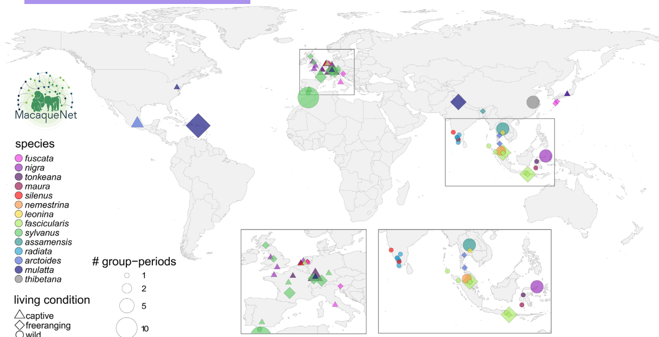
FIGURE 2 Geographical distribution of research sites in which the data currently present in the MacaqueNet database have been collected. Populations in America and Europe (with the exception of Gibraltar) have been introduced. Living conditions are classified as wild, free-ranging or captive (see glossary at https://macaquetnet.github.io/documentation/ for definitions). Group-periods represent the total number of study periods for all groups at a given research site.
