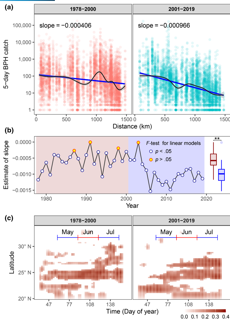
FIGURE 4 The migration distance of BPH has decreased. Parts (a) and (b) show the relationship between 5-day BPH catches at each of the 229 stations along the migration route and the distance from the hypothetical start point of the migration (Liuzhou City, 109.75°E, 24.30°N, in the NSC region). (a) The relationship between BPH catches and distance from Liuzhou in each time period. In 1978–2000, the linear model (blue line) had a shallower slope than in 2001–2019, indicating that BPH migrated further in the first period than the second period. In the general additive model (black line), there was a peak around the migration distance of 1000 km in the first period, corresponding to the LYRV that was absent in the second period. (b) The slope values of the fitted linear model from (a) but built separately for each year. The slopes were typically steeper in each year from 2001 onwards, and the overall mean values were significantly steeper in the second period than in the first period. (c) Latitude date cross-section of the relative 2-D binned kernel density of the 341 trapping stations (relative density of traps per unit of latitude for each 5-day period) in a BPH concentration zone, based on the data from more than 300 county plant protection stations between 1978 and 2019. Any given BPH trapping station in any 5-day period was defined as a planthopper 'concentration and landing zone' if the number of BPH in the 5-day catches was greater than or equal to the BPH90th (i.e., the 90th percentile value in that period of that year).
