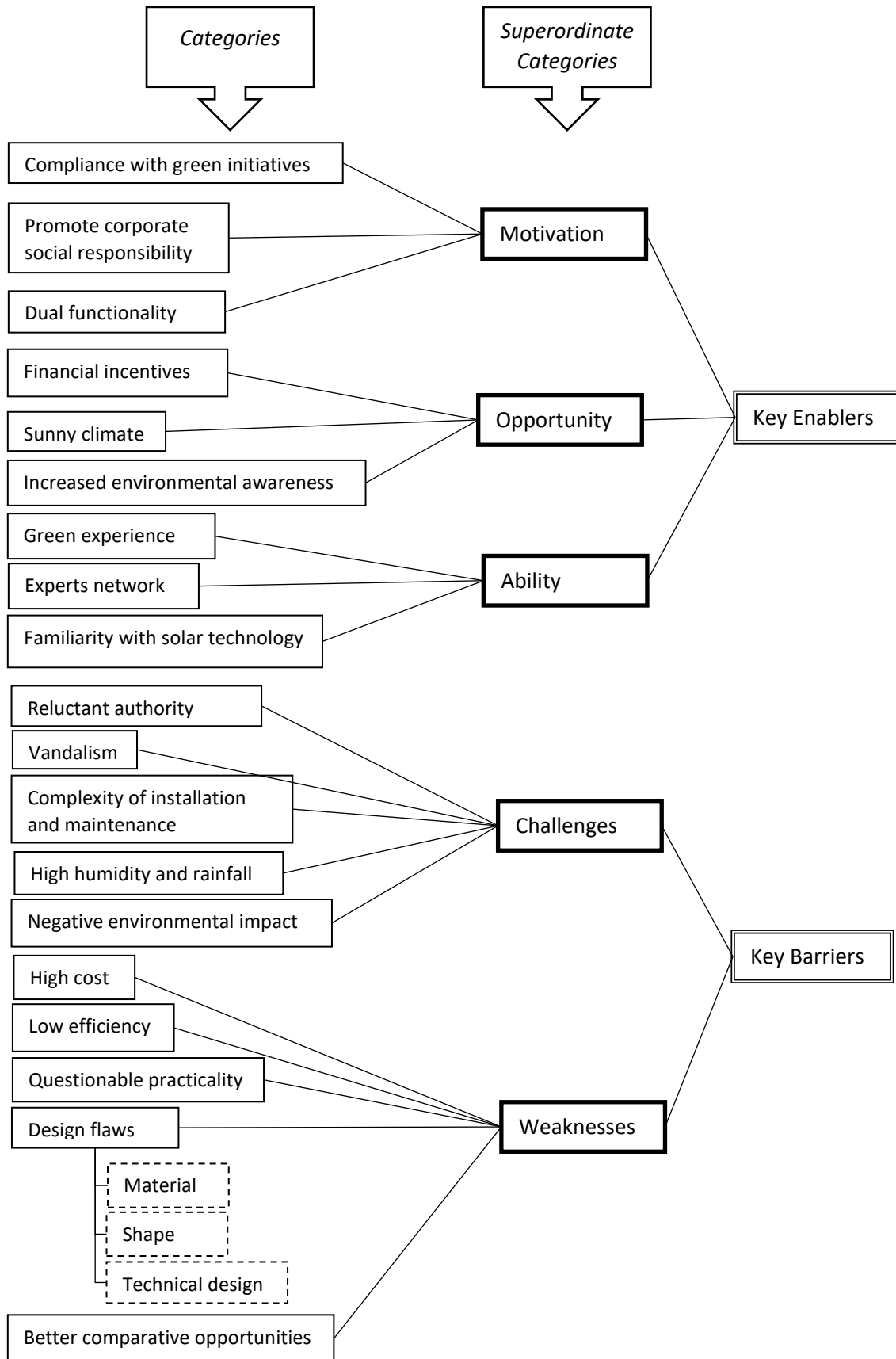
Figure 3. Data Structure
