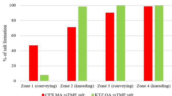
Fig. 7. Transformation kinetics of CFX - MA (red) and KTZ - OA (green) salts in the extrusion segments.
