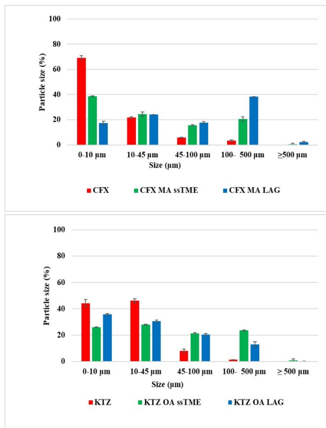
Fig. 4 Particle size distribution of bulk materials and salts synthesised by ssTME and LAG.
