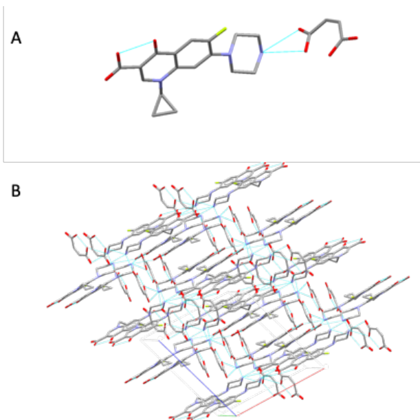
Fig. 2 (A) Interaction between the CFX and MA molecules via dual N+ - HO hydrogen bonds (B) Crystal packing projections for CFX - MA salts. Other hydrogen and Van der Waals bonds have been omitted for clarity.
