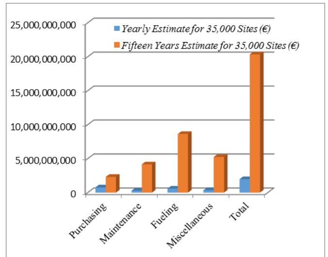
Fig.4. Estimated cost for diesel generator base station for 35,000 sites.
