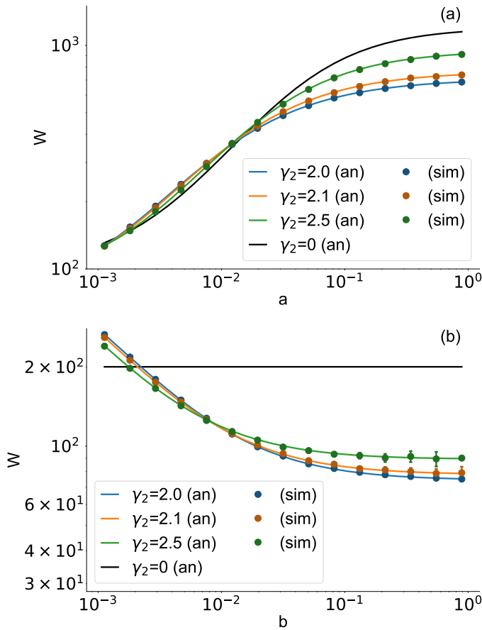
FIG. 4: Stationary state of the random walk process. The average number of walkers per node of class a (a) and b (b) computed analytically (continuous lines) and through numerical simulations (dots) for different values of exponent of the attractiveness distribution \gamma_2 . Error-bars are standard deviations obtained by averaging across 10^3 different network configurations. In the above panel, they are not visible on the scale of the graph. We considered N = 10^5 , m = 6 , W/N = 200 , and \gamma_1 = 2 . The black line shows the case where b_i = 1/N for all nodes.
