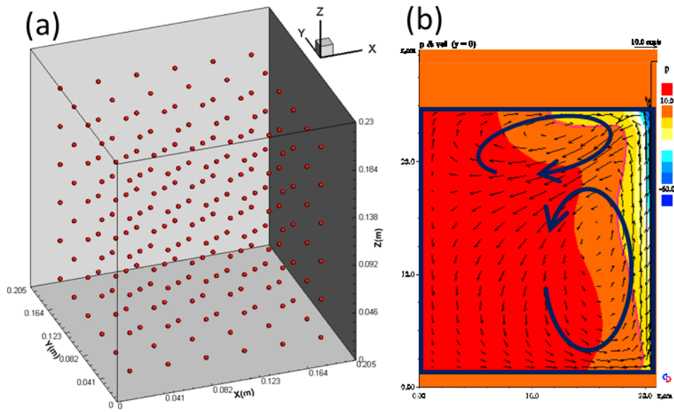
Figure 6 (a) Initial distribution of 216 particle (not to scale) located in the nodes of a 6 \times 6 \times 6 mesh within a cuboid domain of 20.5 \times 20.5 \times 23\ \text{cm}^3 (b) fluid pressure contours and velocity vectors in a 41 \times 41 \times 23\ \text{cm}^3 crucible; quarter of the crucible is shown, assuming symmetry conditions with respect to YZ and XZ planes, large arrows schematically indicate the sense of poloidal motion caused by EM stirring.
