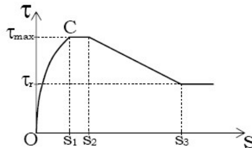
Figure 16. Bond-stresses versus slip for the deformed bar – confined concrete contact behavior according to the Eligehausen model (Eligehausen et al., 1986)
