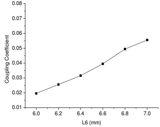
Fig. 7 The variation of the coupling coefficient with the length of the slot.
