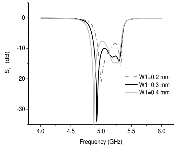
Fig. 11 The variation of the bandwidth with W1.
