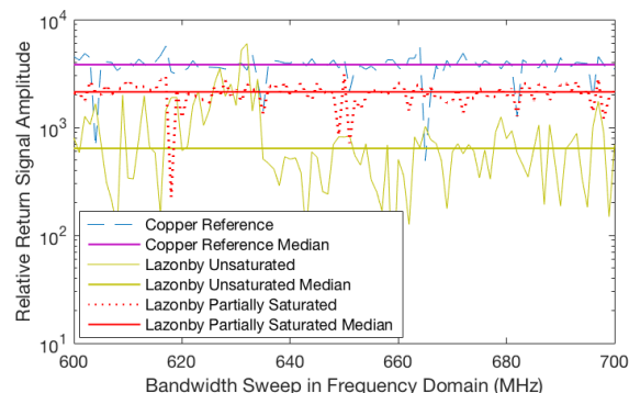
FIGURE 9 Return signal amplitudes for room-dry and partially water saturated Lazonby sandstone, with copper sheet acting as an ideal reflector, and with data medians indicated over a 100 MHz sample size (between 600-700 MHz bandwidth sweep, see Figure 8)
