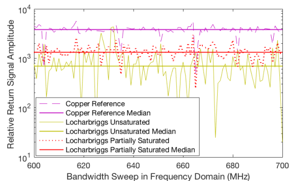
FIGURE 11 Return signal amplitudes for room-dry and partially water saturated Locharbriggs sandstone, with copper sheet acting as an ideal reflector, and with data medians indicated over a 100 MHz sample size (between 600-700 MHz bandwidth sweep, see Figure 10)
