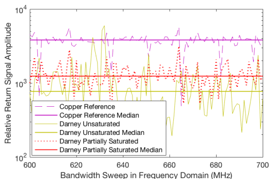
FIGURE 7 Return signal amplitudes for room-dry and partially water saturated Darney sandstone, with copper sheet acting as an ideal reflector, and with data medians indicated over a 100 MHz sample size (between 600-700 MHz bandwidth sweep, see Figure 6)
