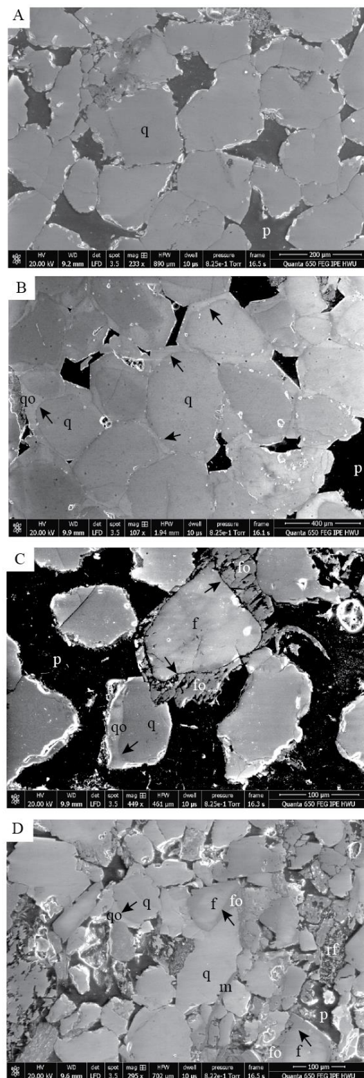
Figure 4 Gaseous secondary electron (GSE) images. A= Darney sandstone, B= Lazonby sandstone, C= Locharbriggs sandstone and D= Red St. Bees sandstone. Key: p = pore, q = quartz, qo = quartz overgrowth, f = feldspar, rf = rotten feldspar, fo = feldspar overgrowth, c = clay, m = mica
