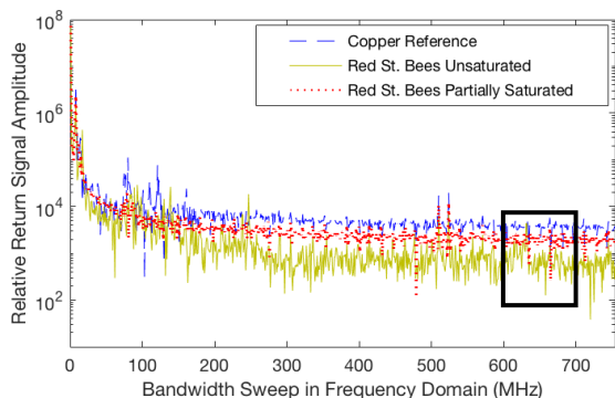
FIGURE 12 Return signal amplitudes, extracted via Fourier transform, for room-dry and partially saturated Red St. Bees sandstone with copper sheet acting as an ideal reflector
