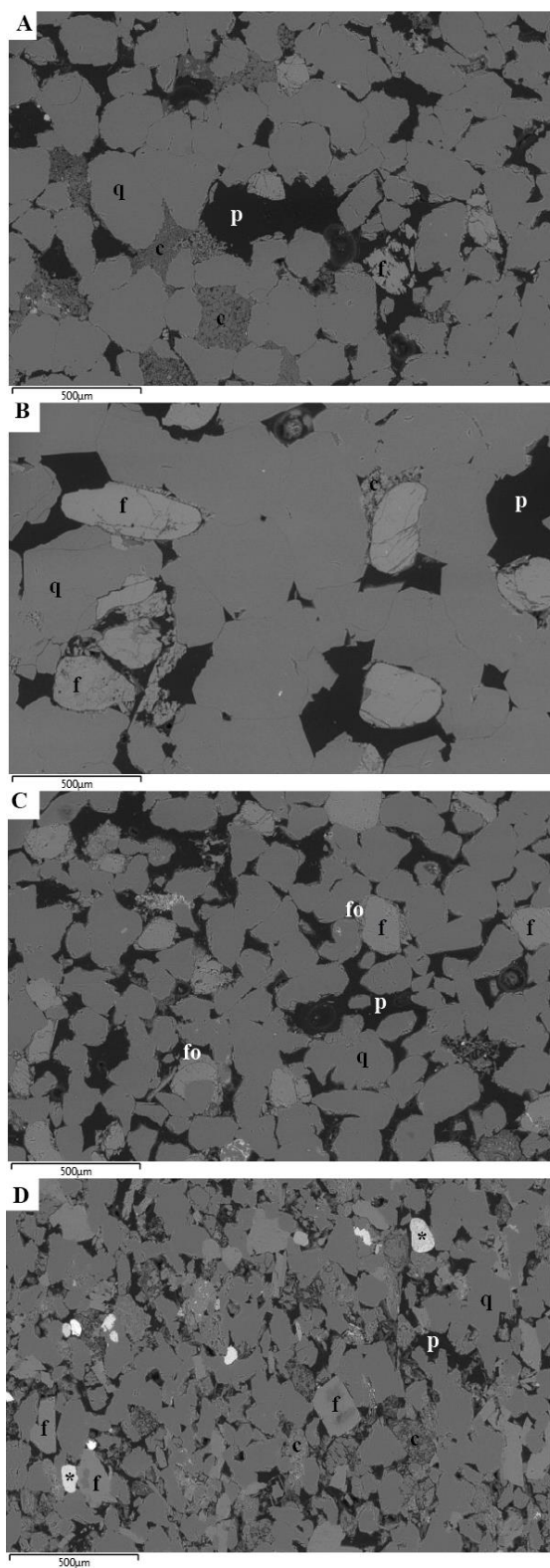
Figure 3 Backscattered electron (BSE) images. A= Darney sandstone, B= Lazonby sandstone, C= Locharbriggs sandstone and D= Red St. Bees sandstone. Key: p = pore, q = quartz, f = feldspar, fo = feldspar overgrowth, c = clay, * = iron-rich particles
