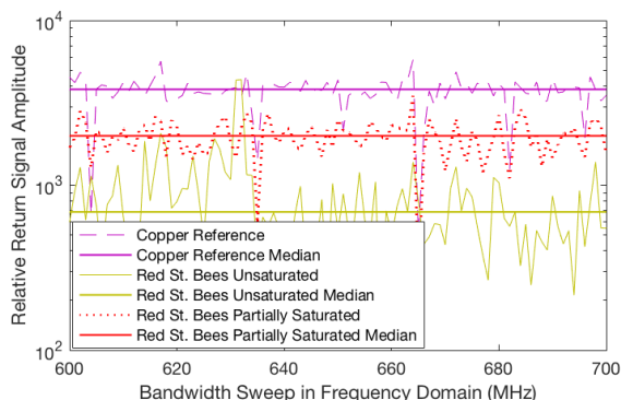
FIGURE 13 Return signal amplitudes for room-dry and partially water saturated Red St. Bees sandstone, with copper sheet acting as an ideal reflector, and with data medians indicated over a 100 MHz sample size (between 600-700 MHz bandwidth sweep, see Figure 12)
