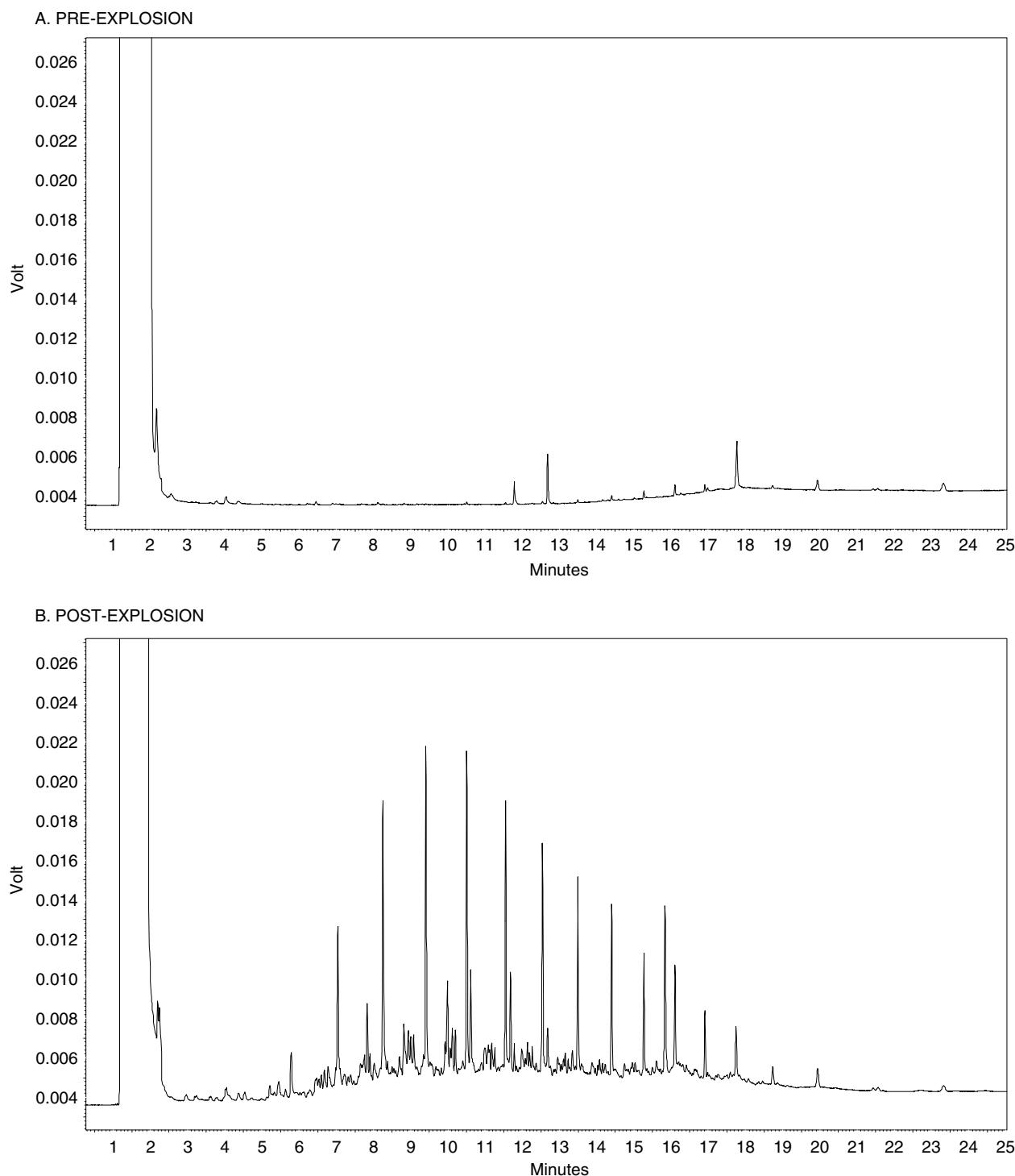
Figure 5. GC-FID chromatograms from soil samples from Kotolname, (A) from a pre-explosion sample and (B) from a post-explosion sample, showing different hydrocarbon peaks, fractions from diesel and petroleum pollution.
