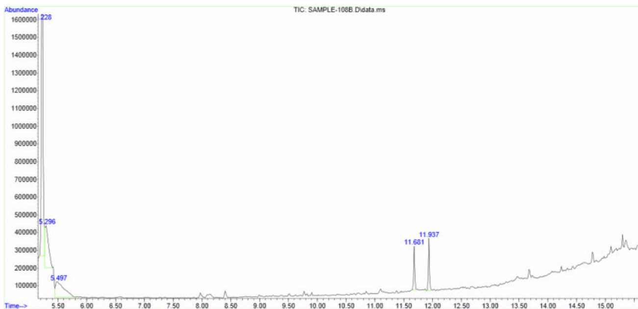
Figure 3. GCMS total ion chromatogram, showing fenitrothion at 11.681 min and fenthion at 11.937 min.
