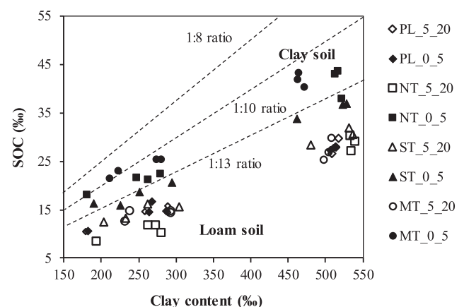
Fig. 7. Clay content and soil organic carbon (SOC) concentration of all the experimental plots ( n = 3 for the clay soil and n = 4 for the loam soil) for the four soil tillage treatments (PL = ploughing, NT = no-till, ST = shallow tillage, MT = minimum tillage) and for two soil depth intervals, i.e., the 0–5 cm and 5–20 cm. The values of the 5–20 cm depth interval are the mean of the 5–10 cm and 10–20 cm depth intervals.
