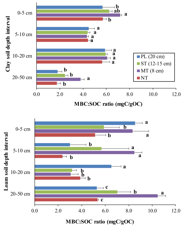
Fig. 6. Mean values ( \pm standard error) of microbial quotient (MicQ), i.e., the ratio between the microbial biomass carbon (MBC) and the soil organic carbon (OC), in the clay ( n = 3 ) and in the loam ( n = 4 ) soil in response to the four tillage treatments along the soil profile. Within each soil depth interval, significant differences among tillage treatments are identified by different superscript letters ( p < 0.05 , Fisher LSD post-hoc test). PL: ploughing (20–25 cm); ST: shallow tillage (12–15 cm); MT: minimum tillage (5–8 cm); and NT: no-till.
