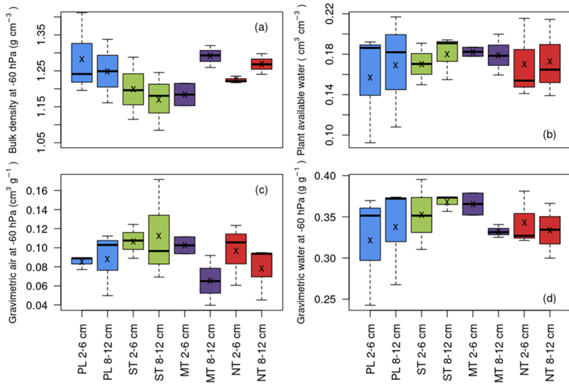
Fig. 8. Boxplots of bulk density (a), plant available water (b), gravimetric air content (c), and gravimetric water content at -60 hPa in the clay soil for the four tillage treatments (PL: ploughing, ST: shallow tillage, MT: minimum tillage, NT: no-till) at two soil depths (2–6 cm and 8–12 cm). Boxplots show mean values (cross), median values (solid horizontal line), 50th percentile values (box outline), minimum and maximum values (whiskers).
