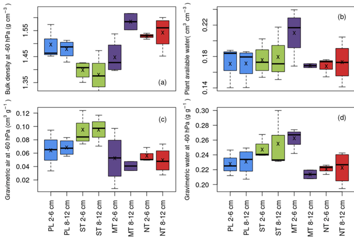
Fig. 9. Boxplots of bulk density (a), plant available water (b), gravimetric air content (c), and gravimetric water content at -60 hPa in the loam soil for the four tillage treatments (PL: ploughing, ST: shallow tillage, MT: minimum tillage, NT: no-till) at two soil depths (2–6 cm and 8–12 cm). Boxplots show mean values (cross), median values (solid horizontal line), 50th percentile values (box outline), minimum and maximum values (whiskers).
