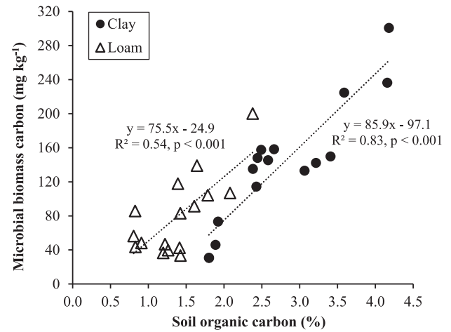
Fig. 4. Linear regression and Pearson's correlation coefficient between the concentration of soil organic carbon (%) and the corresponding amount of microbial biomass carbon ( \text{mgC kg}^{-1} of dry soil) across the four soil tillage treatments at each of the four soil depths. Each value is the mean of three replicates for the clay soil and four replicates for the loam soil.
