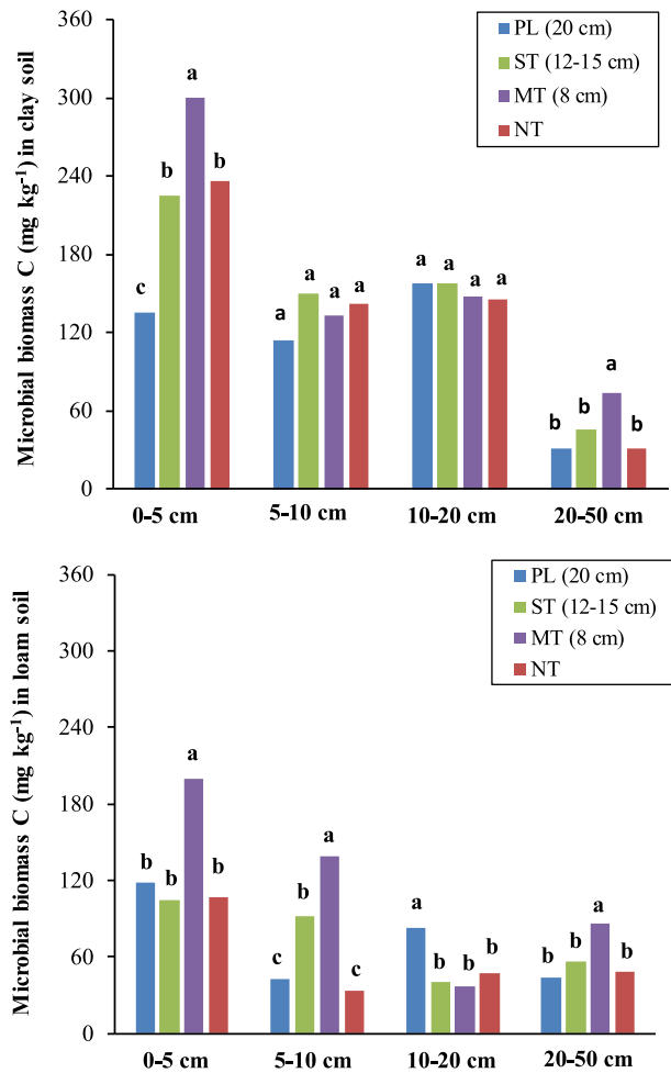
Fig. 5. Mean values of microbial biomass carbon (C) in the clay ( n = 3 ) and in the loam ( n = 4 ) soil in response to the four tillage treatments along the soil profile. Within each soil depth interval, significant differences among tillage treatments are identified by different superscript letters ( p < 0.05 , Fisher LSD post-hoc test). PL: ploughing (20–25 cm); ST: shallow tillage (12–15 cm); MT: minimum tillage (5–8 cm); and NT: no-till.
