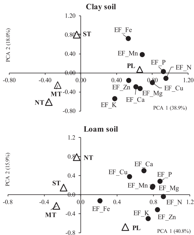
Fig. 2. PCA ordination of the enrichment factors (EF) for macro- and micro-nutrients in winter wheat grains for the clay and the loam soil in relation to the tillage treatments. PL: ploughing (20–25 cm); ST: shallow tillage (12–15 cm); MT: minimum tillage (5–8 cm); and NT: no-till.
