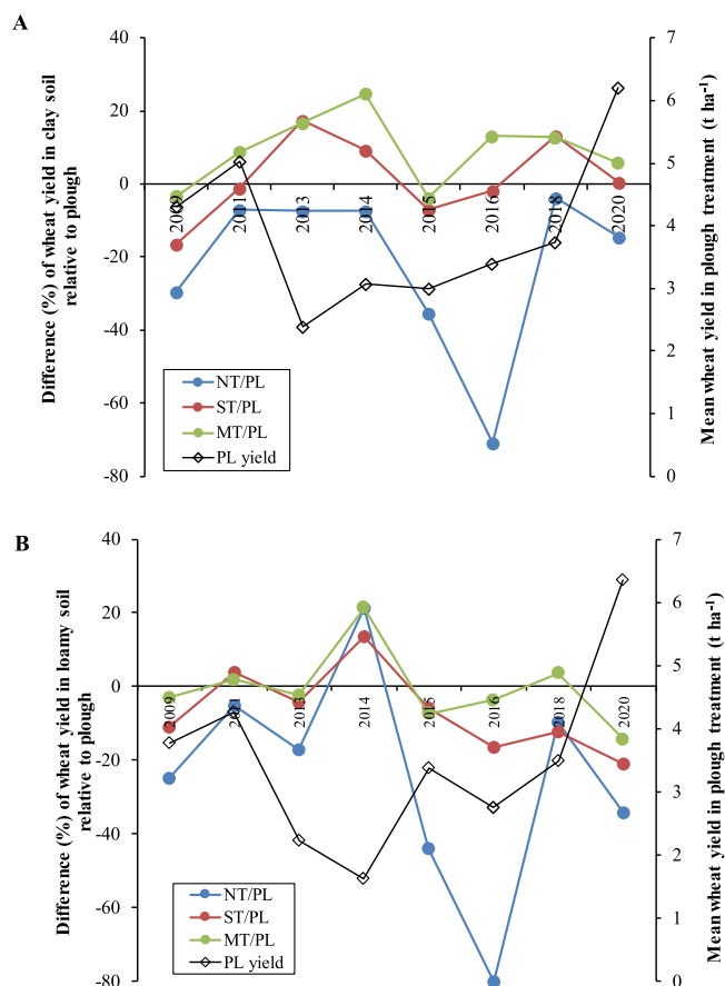
Fig. 1. Temporal trend of the relative difference (%) of the mean winter wheat yield in the no-till (NT), shallow tillage (ST), and minimum tillage (MT) treatment to the mean yield in the conventional ploughing (PL) for the clay (panel A) and the loam (panel B) texture. As reference, the mean yield ( \text{t ha}^{-1} ) in the ploughed treatment is also reported for both soil textures (PL yield).
