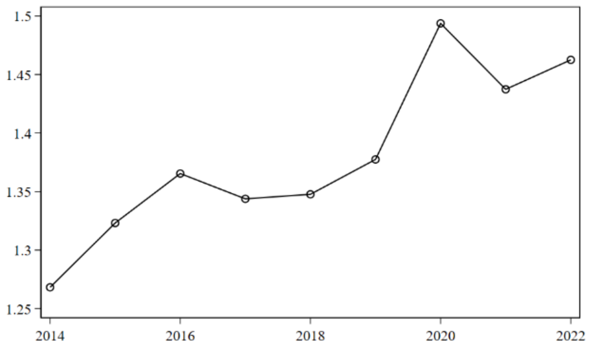
Figure 1: Revenue-weighted average markup in the UK
