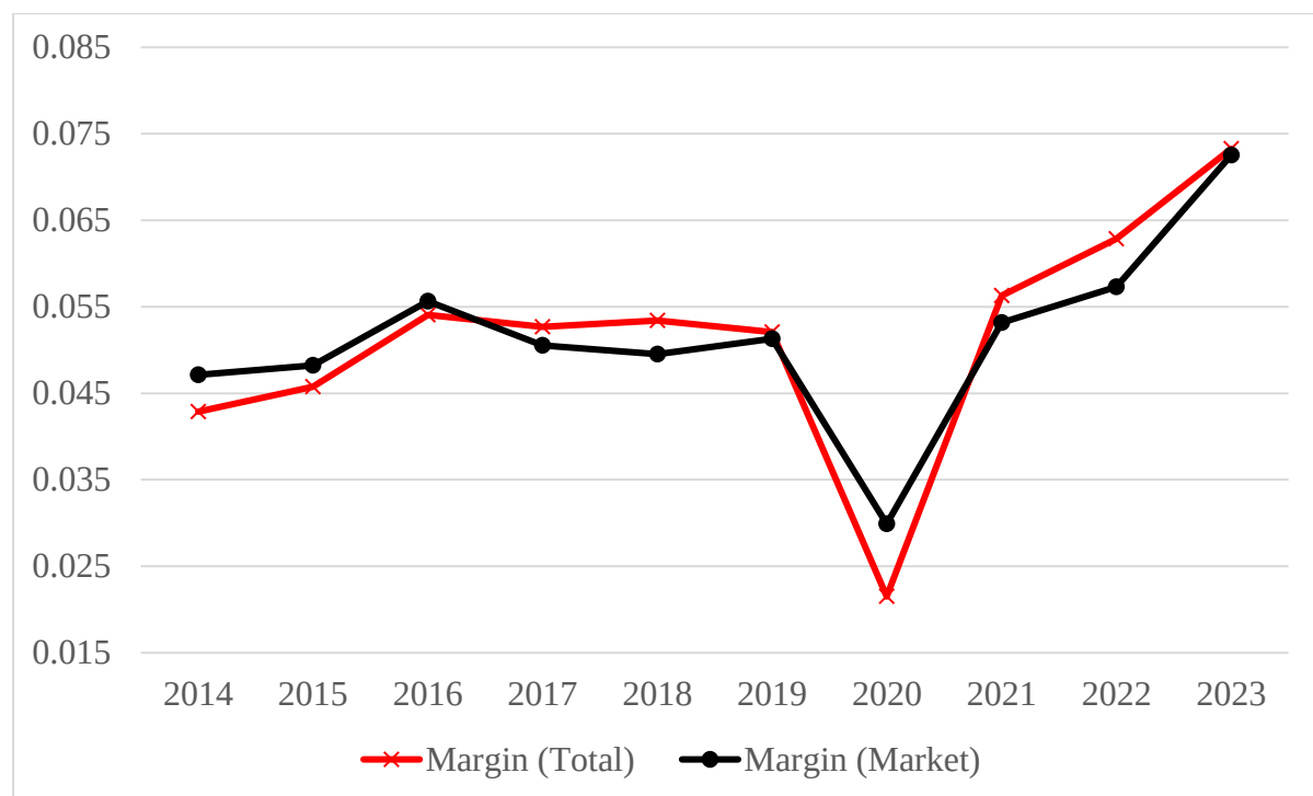
Figure 13: Sales-weighted average profit margin
