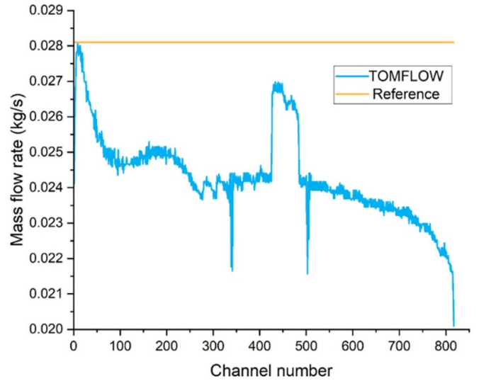
Figure 21. Minimum mass flow rate needed for each channel in the OBC segment.
