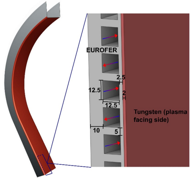
Figure 18. Detail of the FW cooling channels (poloidal-radial section view). The dimensions are indicated in mm. The blue-to-red arrows display the He flow direction.
