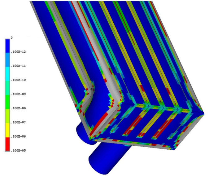
Figure 12. Probability of failure in the bottom region. Case 2.
