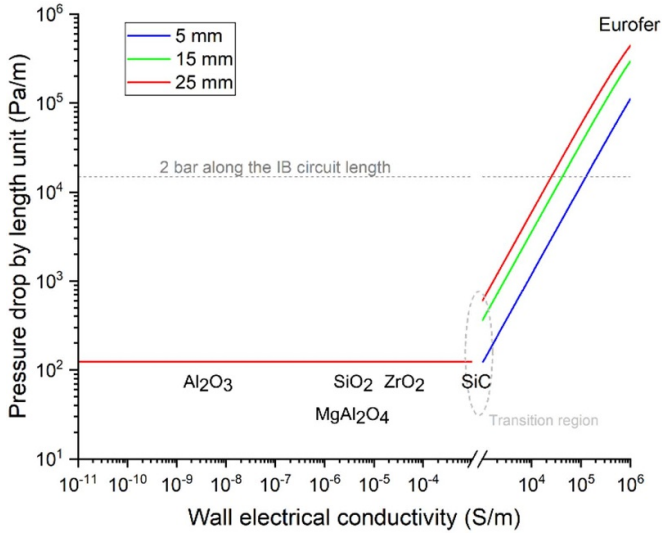
Figure 4. Pressure gradient in the front PbLi channels of the IB segments for a range of wall electrical conductivity (taken at representative T \sim 550^\circ\text{C} – 650^\circ\text{C} ) and three values of wall thickness.
