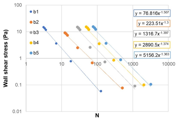
Figure 31. Wall shear stress obtained in the outer side of the samples wall in function of the Stuart number ( N ).
