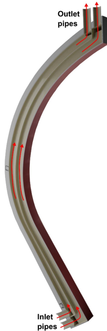
Figure 1. Radial-poloidal section view of the outboard central segment. PbLi paths indicated by red arrows.
