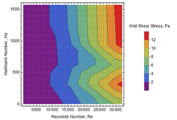
Figure 30. Wall shear stress as a function of Re and Ha in the outer wall line.
