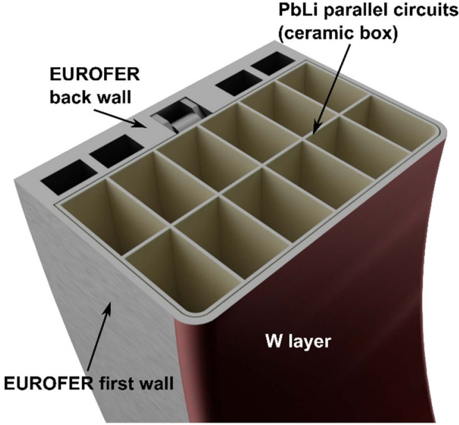
Figure 2. Radial-toroidal section view of the outboard central segment.
