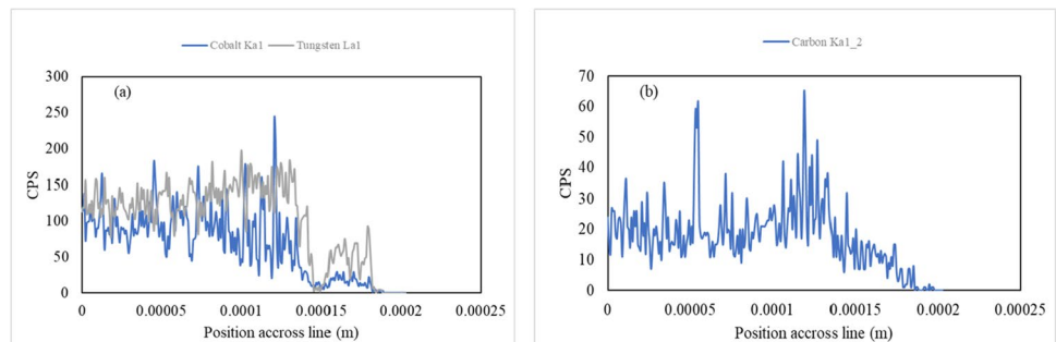
Fig. 10 Reduction in the percentage of cobalt and tungsten (a) and carbon (b) from the tool surface
