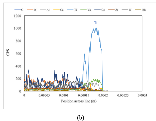
Fig. 6 a SEM micrograph showing the elemental mapping performed using line scan analysis. b Elemental mapping performed on the used insert with counts per second (CPS) against the position across the line
