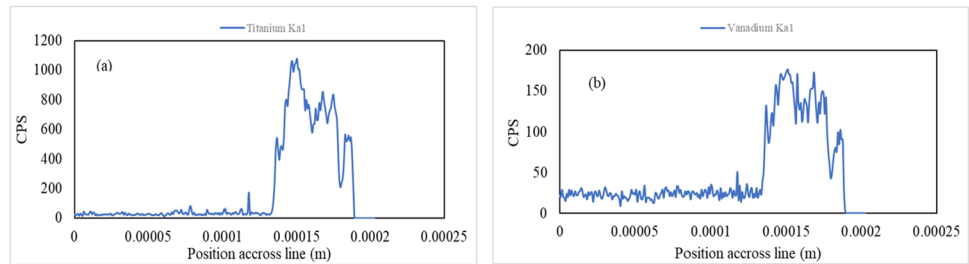
Fig. 8 Increase in adhesion of titanium (a) and Vanadium (b) on the flank face
