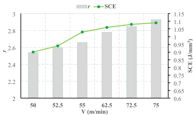
Fig. 13 Effect of chip compression on SCE at different cutting speeds
