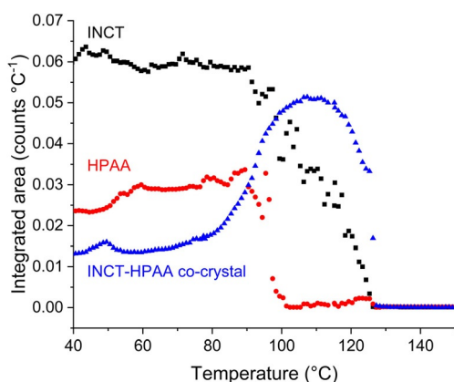
Figure 8. Plot of relative quantity as a function of temperature for each of the phases present in a mixture of INCT and HPAA.
