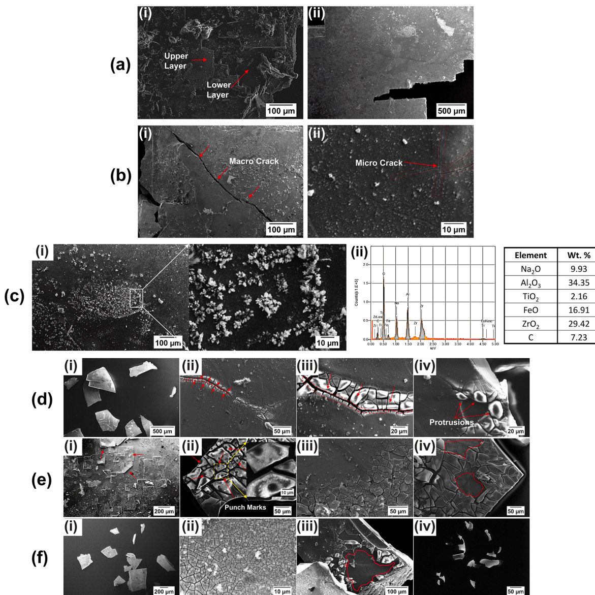
Fig. 6. (a) SEM images of an extracted Al 3 Zr crystal showing layered and faceted morphology, (b) presence of pre-existing micro-cracks, and (c) oxides and the EDS spectrum with elemental composition. (d) SEM morphological images of cavitation damage induced after 3 sec, (e) 6 sec, and (f) 9 sec sonication, obtained at ultrasonic amplitude of 210 \mu m peak-to-peak.
