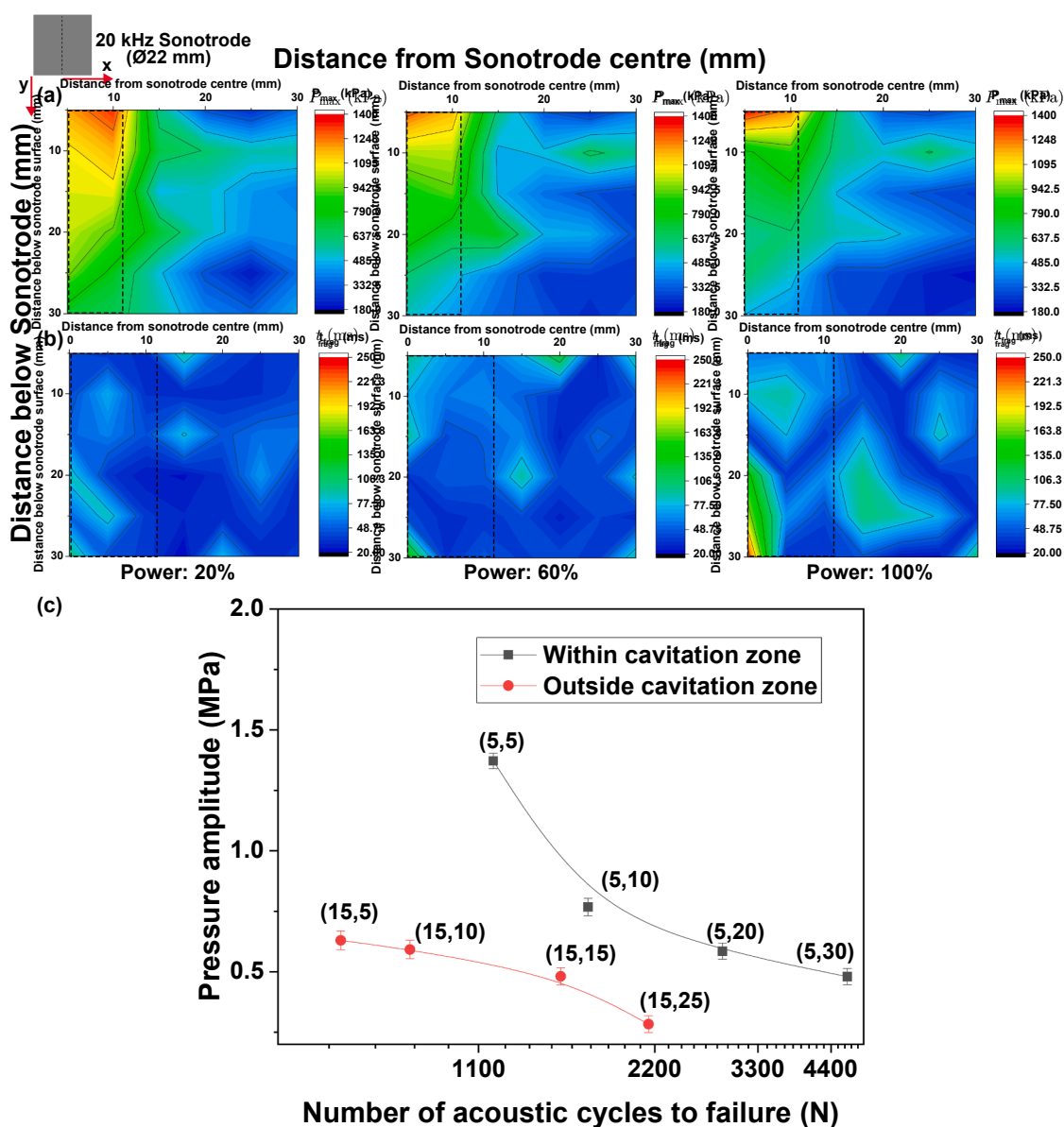
Fig. 2. Contour plots of (a) effective treatment domain with maximum pressure ( P_{\text{max}} ) distribution obtained from NH, (b) fragmentation time of fixed intermetallic crystals, obtained at 20%, 60% and 100% input power. (c) Variation of cyclic pressure amplitude with respect to the acoustic (sonotrode motion) cycles to failure of the crystal measured from the onset of cavitation activity at 100% input power at (x, y) position in mm away from the horn.
