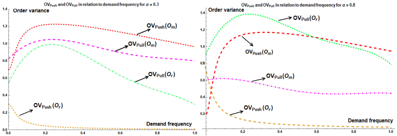
Fig. 5. Order variance of O_r and O_m in relation to \omega under \alpha = 0.3 and 0.8 .
