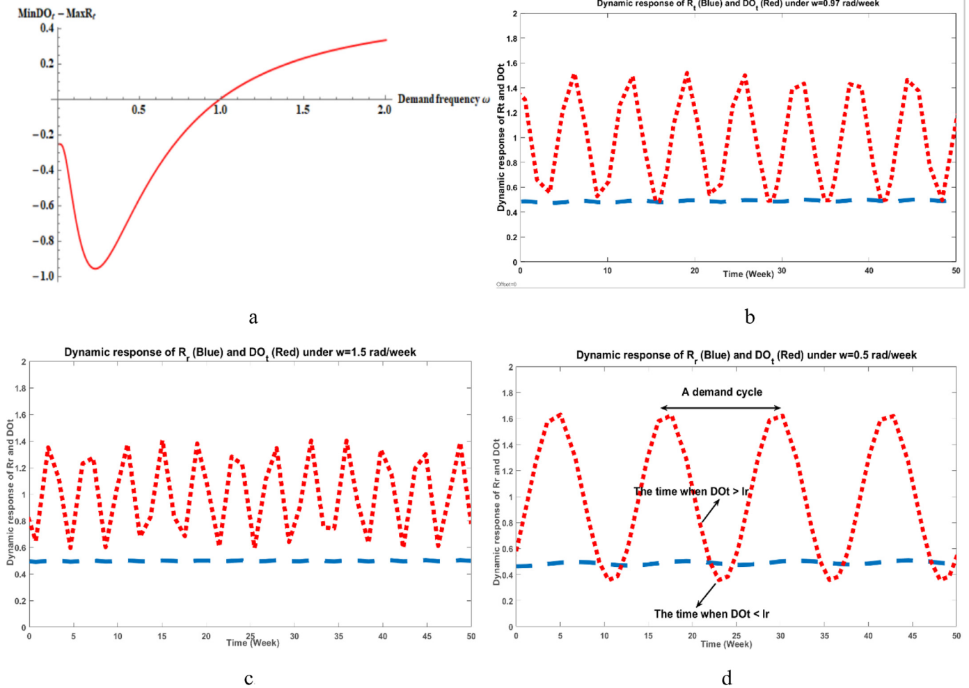
Fig. 3. The plot of \text{MinDO}_t - \text{MaxR}_t as the function of \omega and the dynamic response of \text{DO}_t and R_t under \text{MinDO}_t - \text{MaxR}_t=0 (Fig. 3b), \text{MinDO}_t - \text{MaxR}_t>0 (Fig. 3c) and \text{MinDO}_t - \text{MaxR}_t<0 (Fig. 3d).
