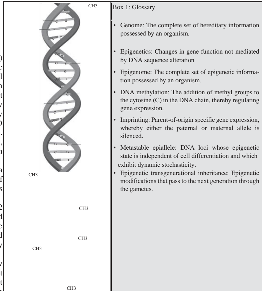
Fig. 1. DNA methylation.
