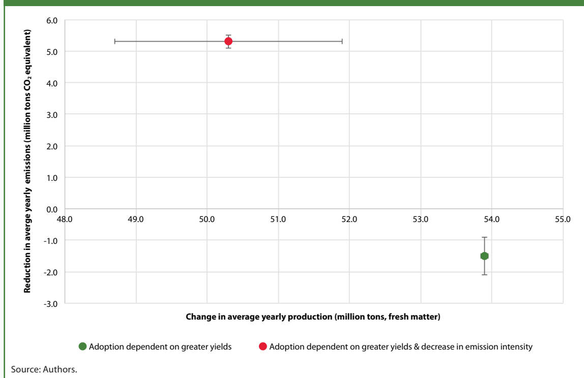
FIGURE 3.5—EFFECTS OF ADOPTION OF THE BEST CLIMATE-SMART AGRICULTURE PRACTICE DURING THE PERIOD 2040–2050 ON TOTAL ANNUAL YIELD AND GREENHOUSE GAS EMISSIONS
