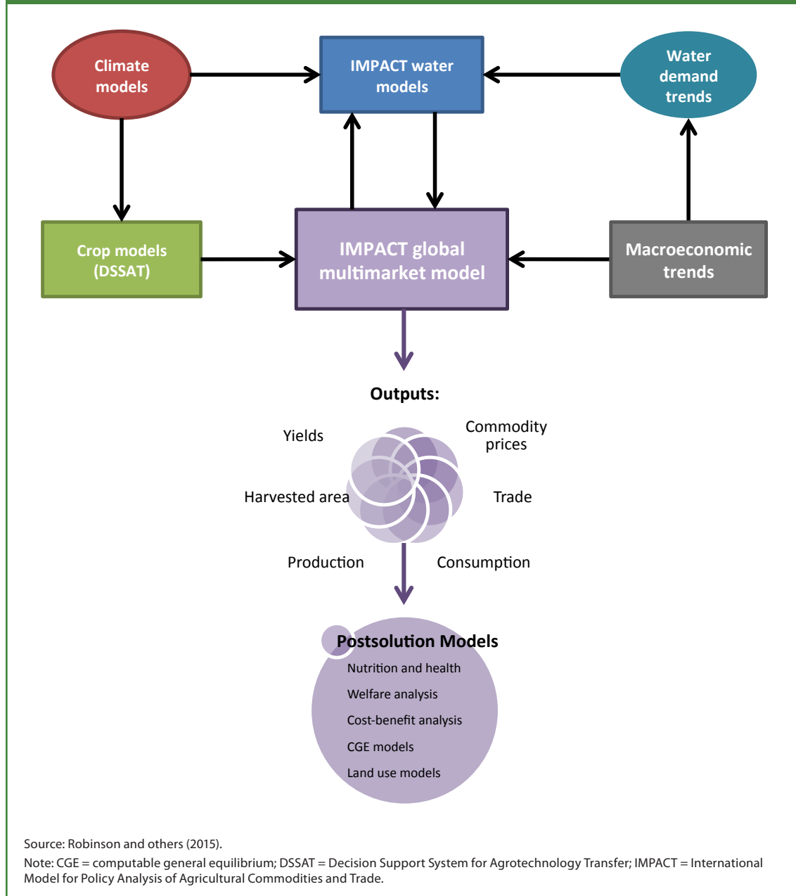
FIGURE 2.7—THE IMPACT SYSTEM OF MODELS
