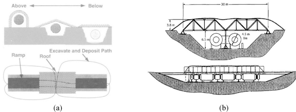
Fig. 11. a) Shielding concepts according to the depth of excavation; b) Large double truss suspends regolith shielding above habitats, Jolly et al. [133].
