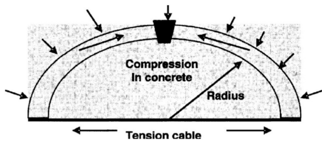
Fig. 16. Wall segment cross section of the proposed arch-shaped structure, Meyers & Toutanji [138].
