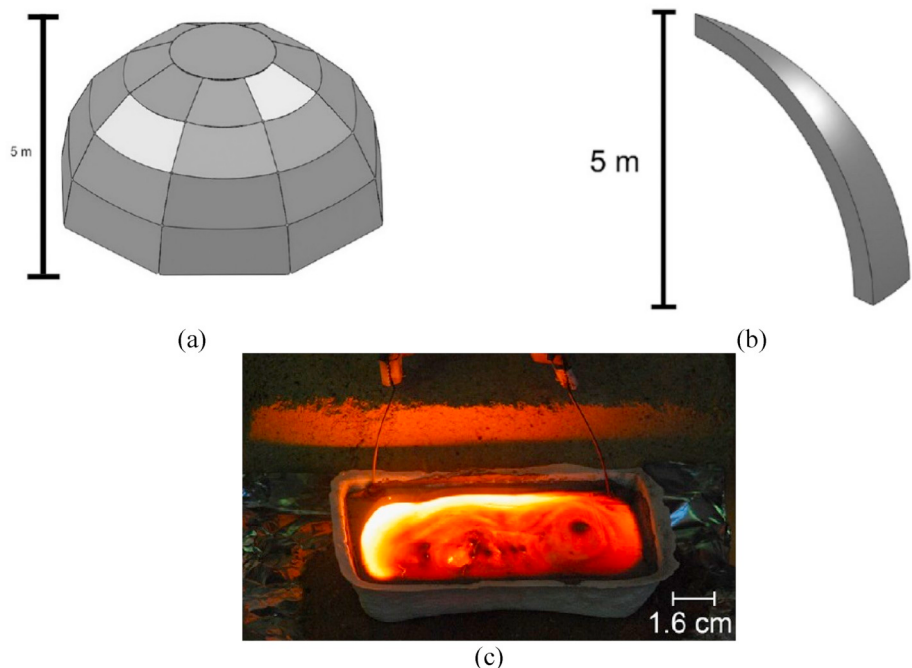
Fig. 17. a) Dome made by regolith-based voussoirs following a geothermite reaction; b) Lune geometry; c) Geothermite reaction using JSC-1A regolith stimulant, Faieron et al. [141].
