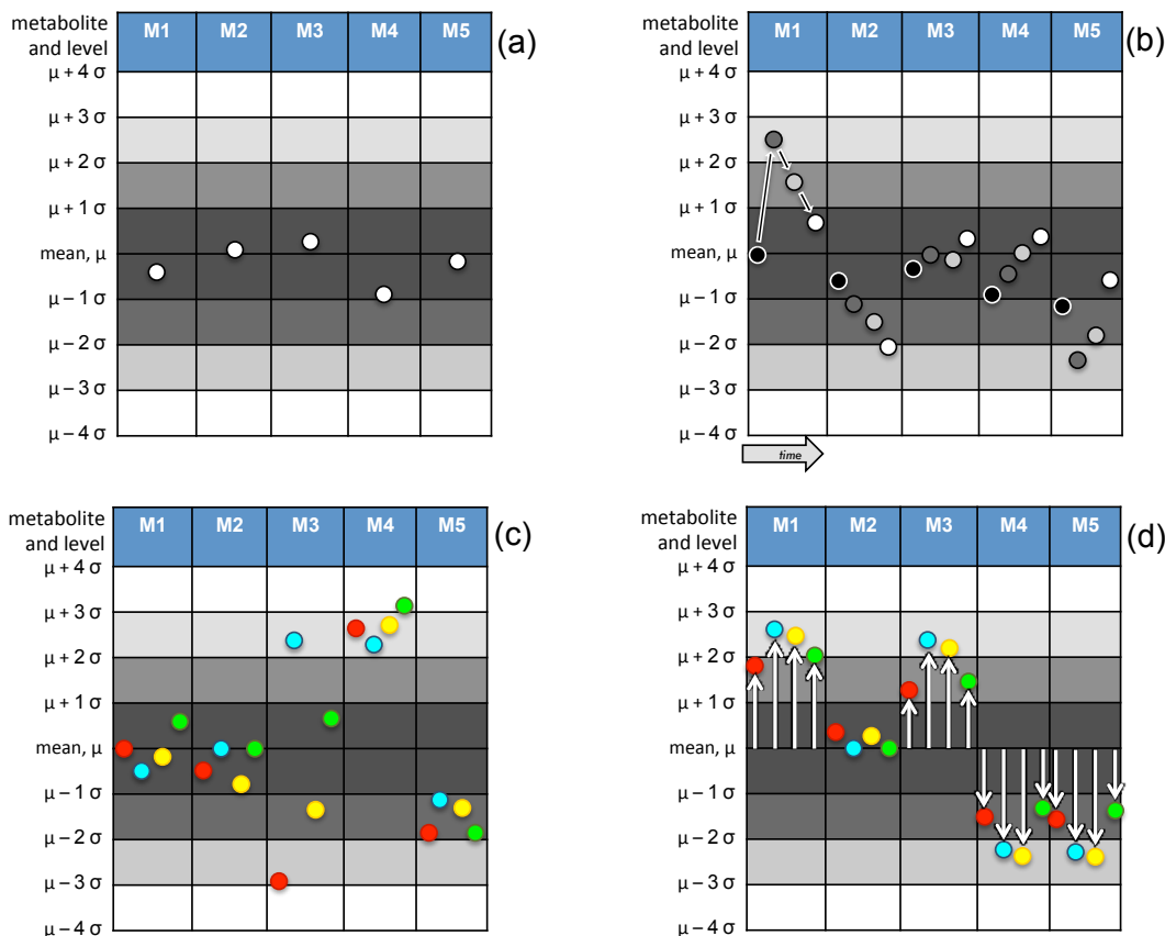
Figure 4. A schematic representation of the four principal approaches to the measurement of metabonomic data: via (a) metabolite levels, (b) trajectories, (c) entropies or (d) correlations/dependencies. In Box (a), the concentrations of 5 different metabolites M1 to M5 in one normal individual (white circles) are superimposed on a chart that represents the normal population distribution of metabolite concentrations. Symbols \mu and \sigma are the mean and standard deviations of the concentrations of the metabolites for that population and with normal distribution. In Box b, we see the trajectories of the concentrations over time for the same 5 metabolites M1 to M5 in one individual subjected to an intervention of some kind. The time course of the metabolic trajectory moves from left to right in each metabolite column and is represented by circles, whose shading gets lighter over time. Arrows connect the time points for metabolite M1 but others are omitted for clarity. It can be seen that as a result of the challenge, the levels of some metabolites (M1, M2 and M5) undergo positive and negative excursions from the normal population values, whereas other metabolites are less affected. In Box (c), the metabolic entropies of a cohort of four individuals that have been subjected to a challenge are represented. The metabolite concentration for each individual is colored differently (red, blue, yellow and green circles represent individuals 1, 2, 3 and 4 respectively). It can be seen that in this cohort there is high metabolic entropy for metabolite M3 (metabolite concentrations are distributed across a very wide range of values/ configurational states following the intervention) and significant disturbances in the metabolite concentrations for M4 and M5, but much lower metabolic entropy or disorder, for metabolites, M1, M2, M4 and M5. In Box (d), the metabolite correlations seen for 5 metabolites (M1 to M5) in 4 human subjects (red, blue, yellow and green circles represent individuals 1, 2, 3 and 4 respectively) are shown following an intervention. The intervention causes a significant increase in the concentrations of metabolite M1 for all four subjects (white vertical arrows), although to differing degrees. The
