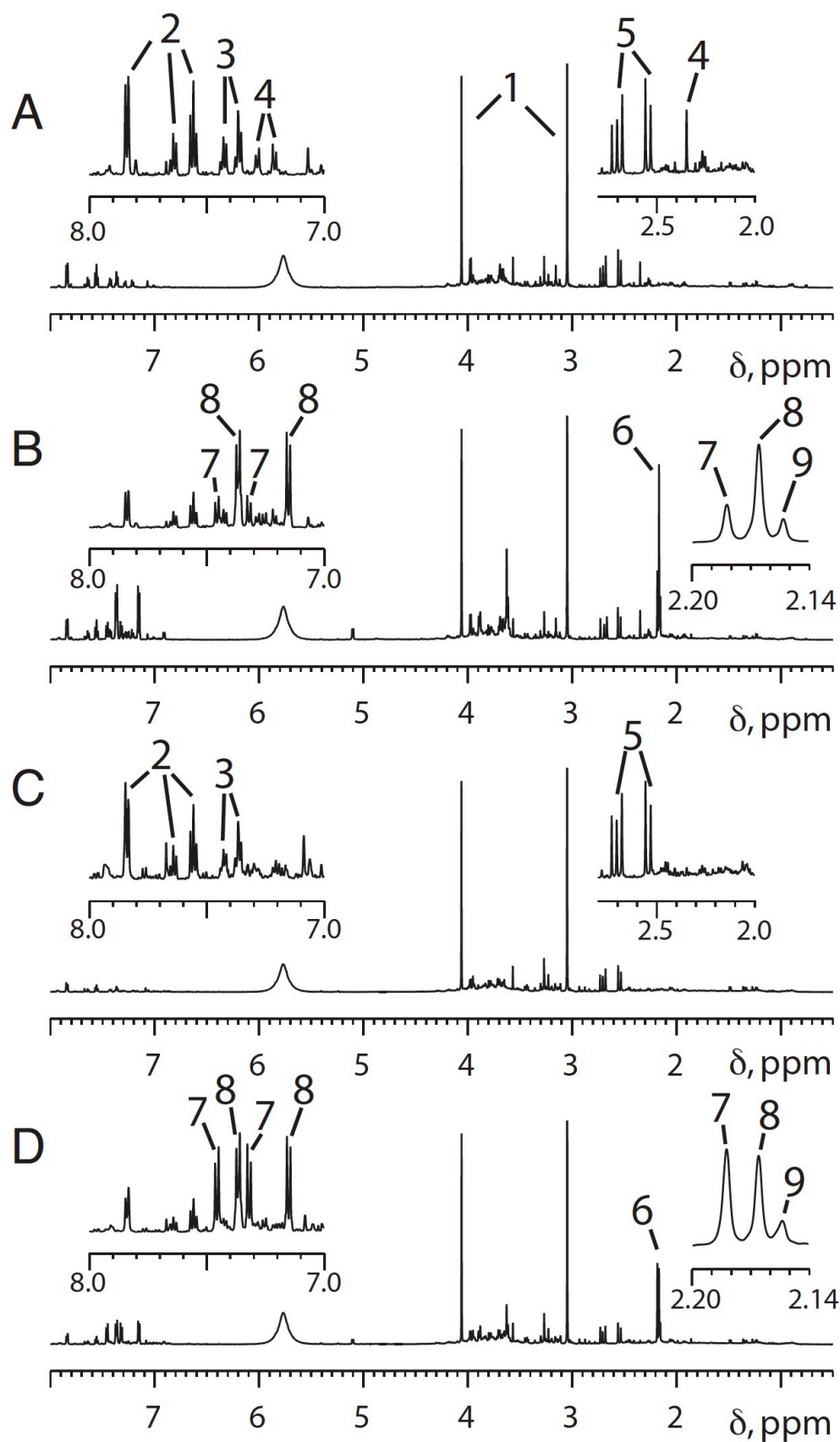
Figure 7: 600 MHz ^1\text{H} NMR spectra of the urines of volunteers taking a 1 g oral dose of paracetamol. A. spectrum of pre-dose urine of volunteer 1 together with expansions of the aromatic and lower frequency regions. B. 0-3 hour post-
