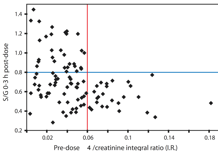
Figure 8: the urinary ratio of paracetamol sulphate (S) to paracetamol glucuronide (G) excreted 0 - 3 hours post-dose plotted against the pre-dose ratio of metabolite 4 normalised to creatinine. Reproduced with permission from PNAS.(Clayton et al. 2009)
