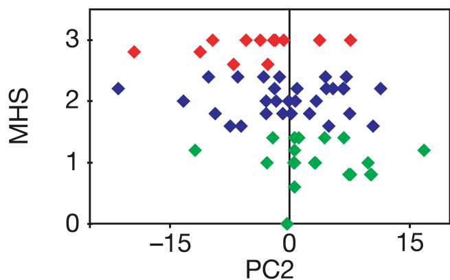
Figure 6: a plot of paracetamol liver toxicity as measured by the mean liver histopathology score (MHS) against principal component 2 (PC2) of the pre-dose urine NMR spectral data. A partial class separation is observed. Each point represents a single rat and is colour-coded by its histology class with increasing degree of liver pathology: class 1 is green (minimal / no pathology), class 2 is blue (intermediate pathology), class 3 is red (significant pathology). Figure reproduced from Nature Publishing Group (Clayton et al. 2006)
