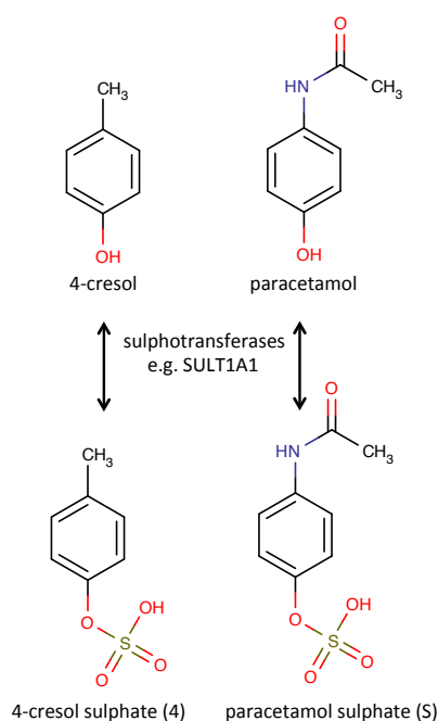
Figure 9: the molecular structures of 4-cresol and paracetamol and their corresponding sulphate metabolites.
