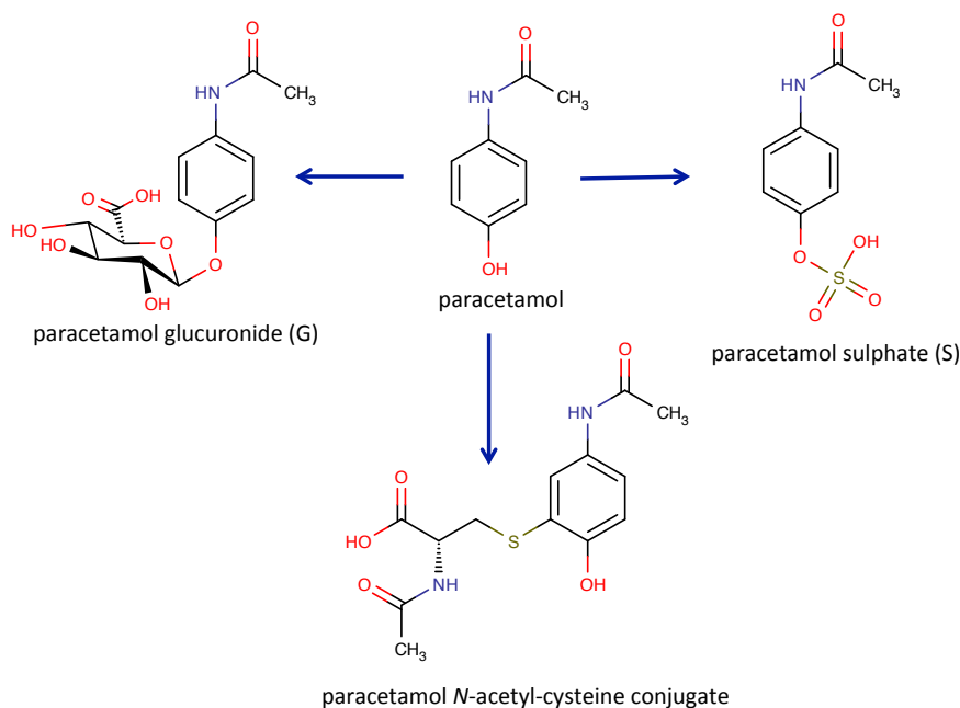
Figure 5: the molecular structures of paracetamol (P) and its major metabolites.
