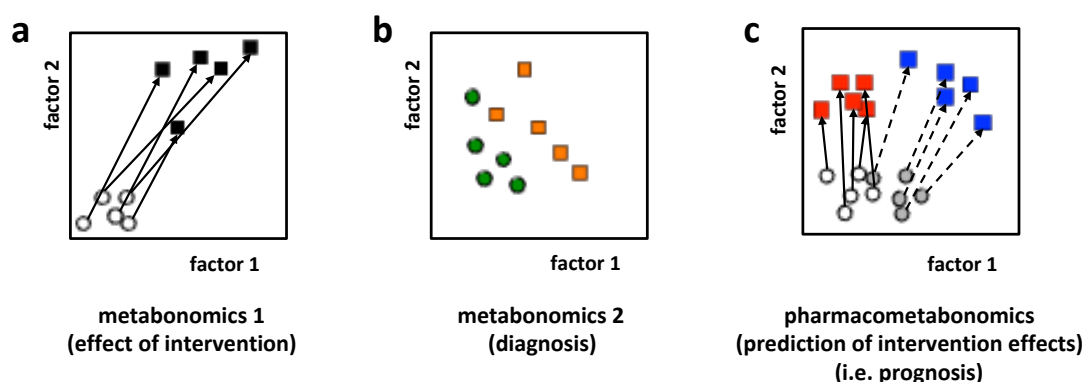
Figure 2. Schematic representations of the outcomes from the two key experimental approaches to metabolic phenotyping, based on multivariate analysis e.g. principal components scores, of the metabolic profiles of a number of individuals and showing the first two components (factor 1 and factor 2). Each square or circle represents an individual subject in the study. a) metabonomics approach 1 (effect of intervention), where open circles represent pre-intervention biofluid metabolic spectral profiles, and black squares represent post-intervention metabolic profiles in the same individuals, where some metabolic perturbation has occurred. The arrows indicate the metabolic trajectory that each individual underwent across metabolic hyperspace as a consequence of the intervention; b) metabonomics approach 2: diagnosis. The metabolite profiles of patients with a disease (orange squares) are distinct from those of healthy controls (green circles) and thus a diagnosis can be made; c) the predictive or prognostic approach. The difference in the pre-intervention metabolic profiles of two sub-groups of subjects (white circles v grey circles) allows prediction of different post-intervention states for
