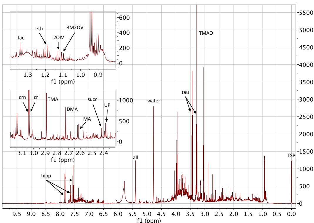
Figure 3. The 600 MHz 1 H NMR spectrum of the urine of a control, male C57BL/6 mouse together with expansions of two low frequency regions, demonstrating the large number of metabolites that can be detected. The identities of some key metabolites are given: 2OIV, 2-oxoisovalerate; 3M2OV, 3-methyl-2-oxovalerate; all, allantoin, cr, creatine; crn, creatinine; eth, ethanol; lac, lactate; DMA, dimethylamine; hipp, hippurate; MA, methylamine; succ, succinate; TMA,
