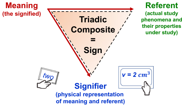
Fig. 1 Data as semiotic representations comprising three composites
