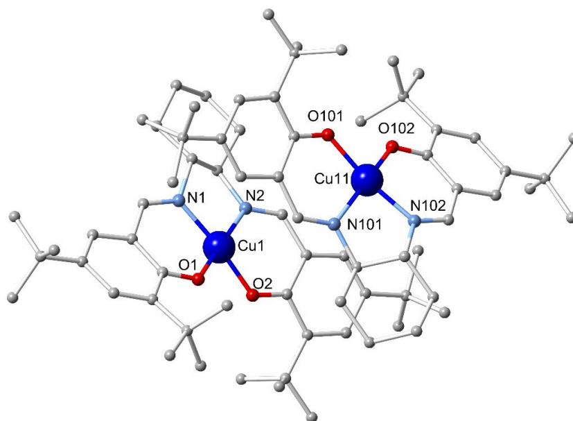
Figure 1. A projection of the asymmetric unit of 1S .
