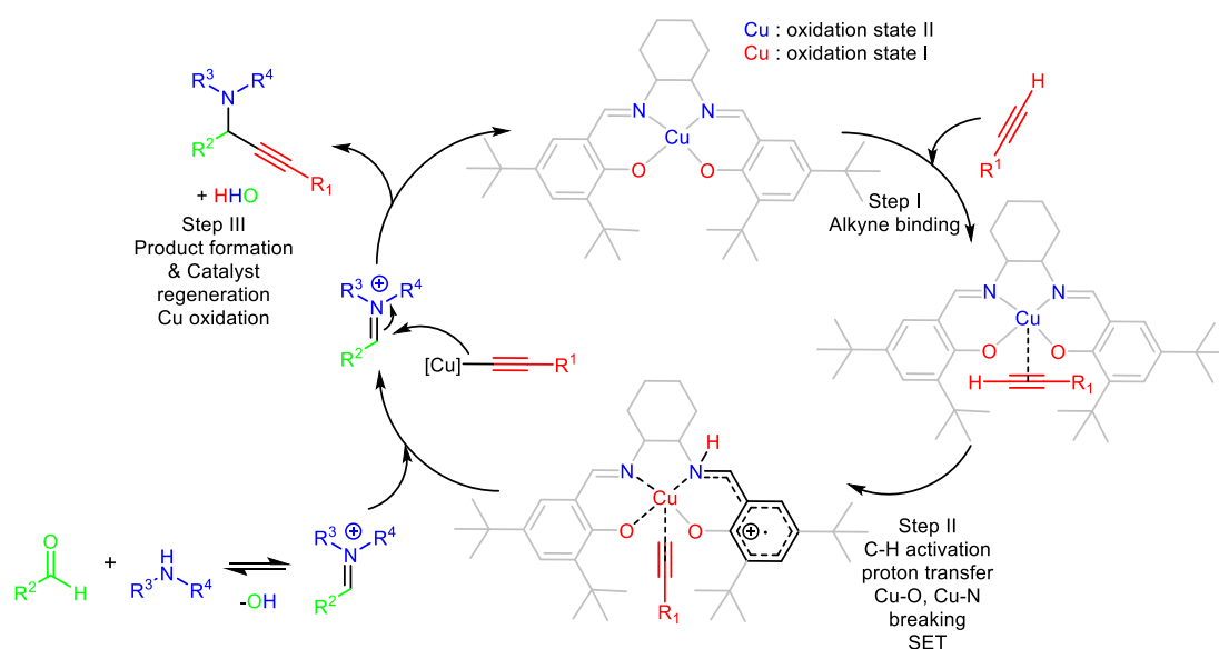
Scheme 2. A plausible mechanism for this reaction.
