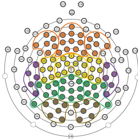
Figure 2. The 128 electrode positions on the scalp. The colors indicate ROIs for left, right, and central regions: orange – frontal, yellow – central, purple – temporal, green – parietal, brown – occipital.
