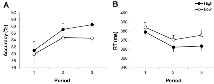
Figure 3. Accuracy (A) and RT for correct responses (B) as a function of period (1-3) and trial type (high- vs. low-frequency triplets). The gap between the curves indicates the statistical learning performance. Error bars denote standard error of mean.
