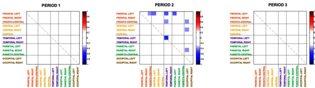
Figure 5. Contribution of theta oscillation (4-7 Hz) functional connectivity to the prediction of overall learning performance measured by accuracy (A) and response time (B). Only significant learning index – functional connectivity correlations are shown separately for periods 1-3 in the matrices between and within the 13 ROIs, respectively. Color bar indicates Pearson's correlation coefficient of the permutation test ( r is scaled between 1 and -1; therefore, red color indicates positive and blue color indicates negative relationship between learning and connectivity).
