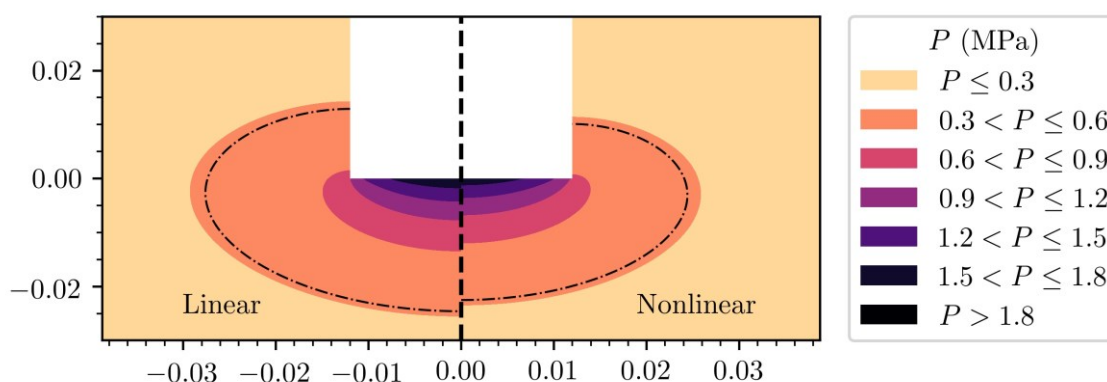
Figure 2. Difference in predicted acoustic pressures between linear and nonlinear models. The nonlinear model includes the attenuating effect of cavitating bubbles below the sonotrode. The dash-dotted line denotes the Blake threshold for hydrogen bubbles in aluminium, with R_0 = 3 \mu\text{m} .
