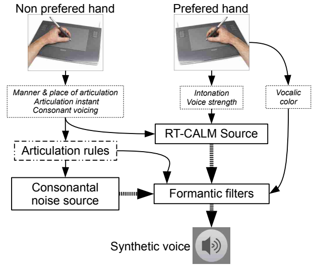
Figure 2: Schematic representation of the Digitartic synthesizer
