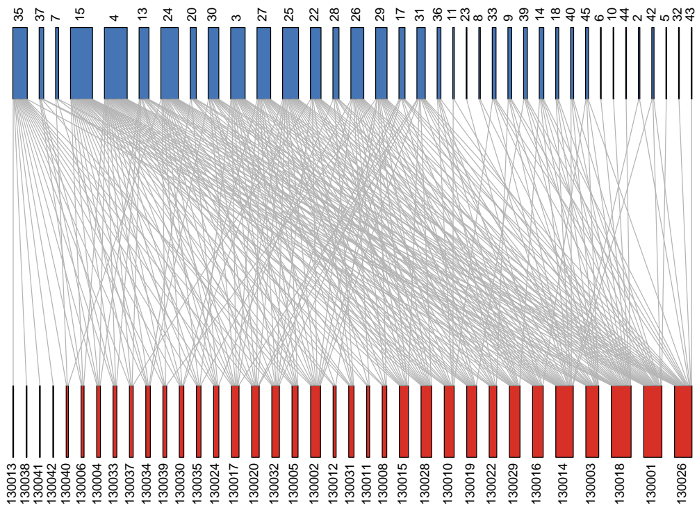
Figure 4: Two-mode network for the year 2003. Red and blue rectangles represent the hospitals and the activities, respectively. Ties indicate which activity belongs to a portfolio of a hospital. The width of a rectangle is proportional to the number of ties incident to that rectangle.
