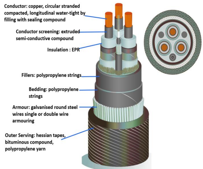
Fig 1. Subsea power cable construction layers [20].
