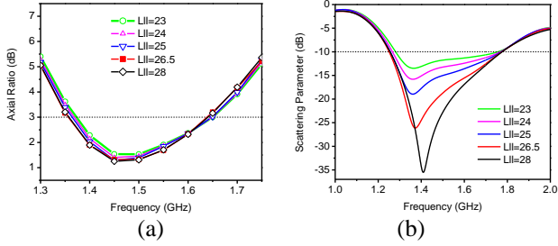
Figure 2: Effect of vertical L-length ( L_{II} ) on (a) AR (b) S_{11}
