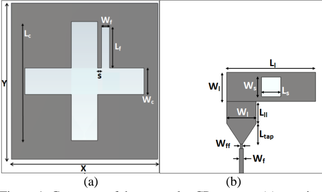
Figure 1: Geometry of the cross-slot CP antenna: (a) top view (b) bottom view. X=75 , Y=80 , L_c=61 , W_c=13.5 , W_f=13.5 , L_l=32 , L_{II}=10.25 , W_{ff}=1.85 , W_{ff}=1 , L_{tap}=10.5 , L_s=9 , W_s=9.25 , L_f=21 , W_f=4 , s=2 (unit: mm)
