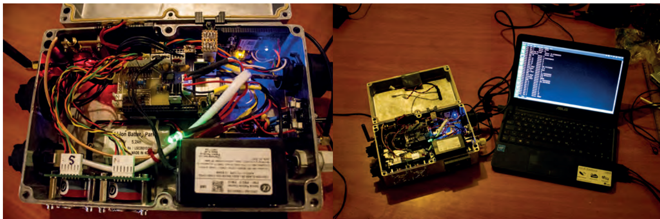
Open design UNEP Air Quality Monitor
