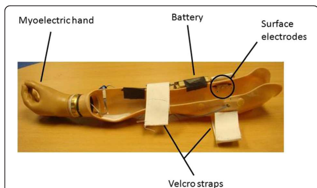
Figure 3 Myoelectric prosthesis simulator. A prosthetic socket which could be fitted over the anatomic arm was produced for every subject. The socket was equipped with a single degree of freedom left sided electrical hand (RSLSteeper "Select" Myo Electric hand (size 3 ¼")), whose opening and closing at a constant speed was controlled via EMG signals from 2 socket-located electrodes.
