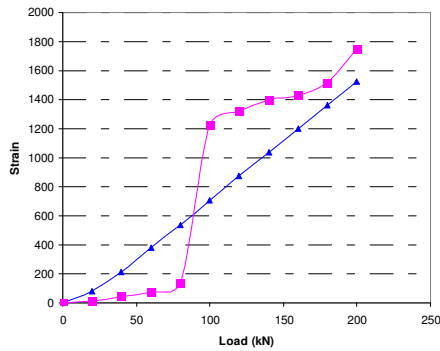
c) Beam NSC2, strain W_i on top of web bar (T12) and tension reinforcement T(20) not yielding.
