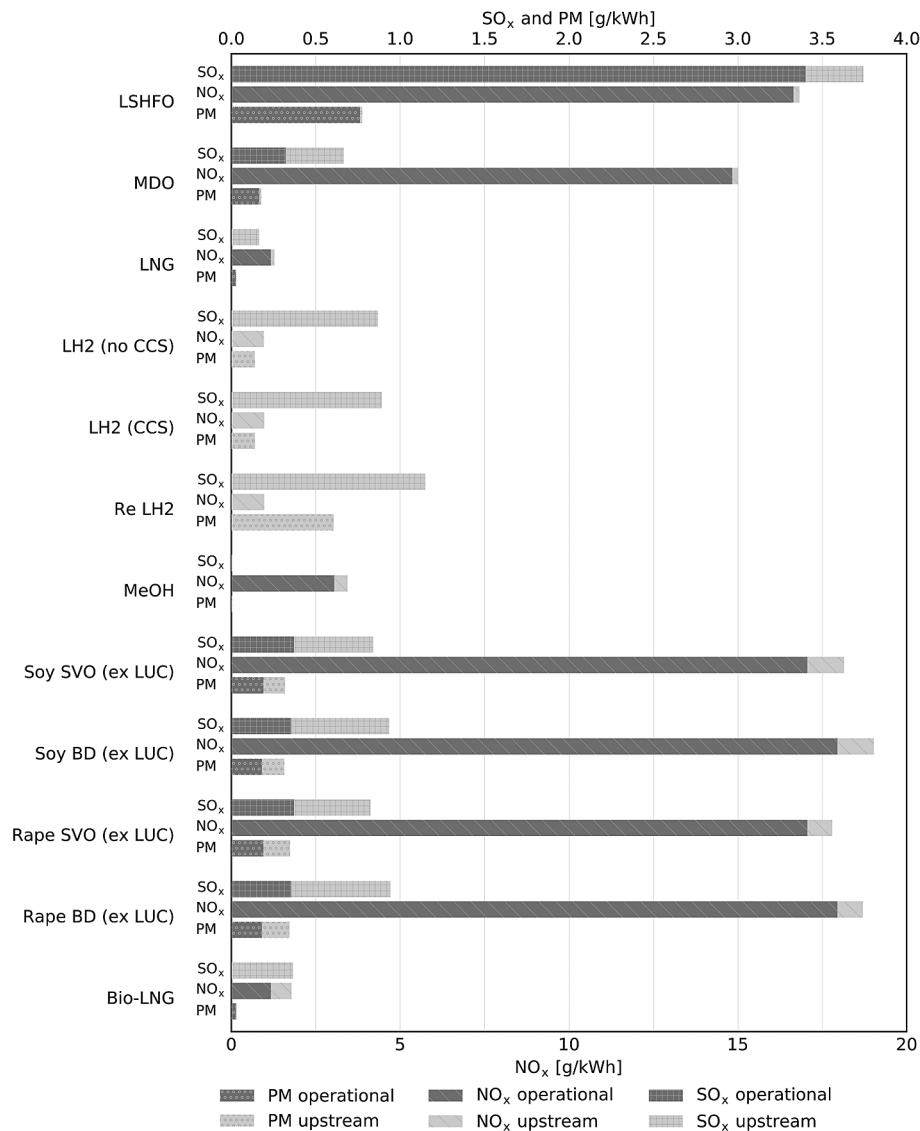
Fig. 4. Non-greenhouse gas emissions per kWh shaft output.
