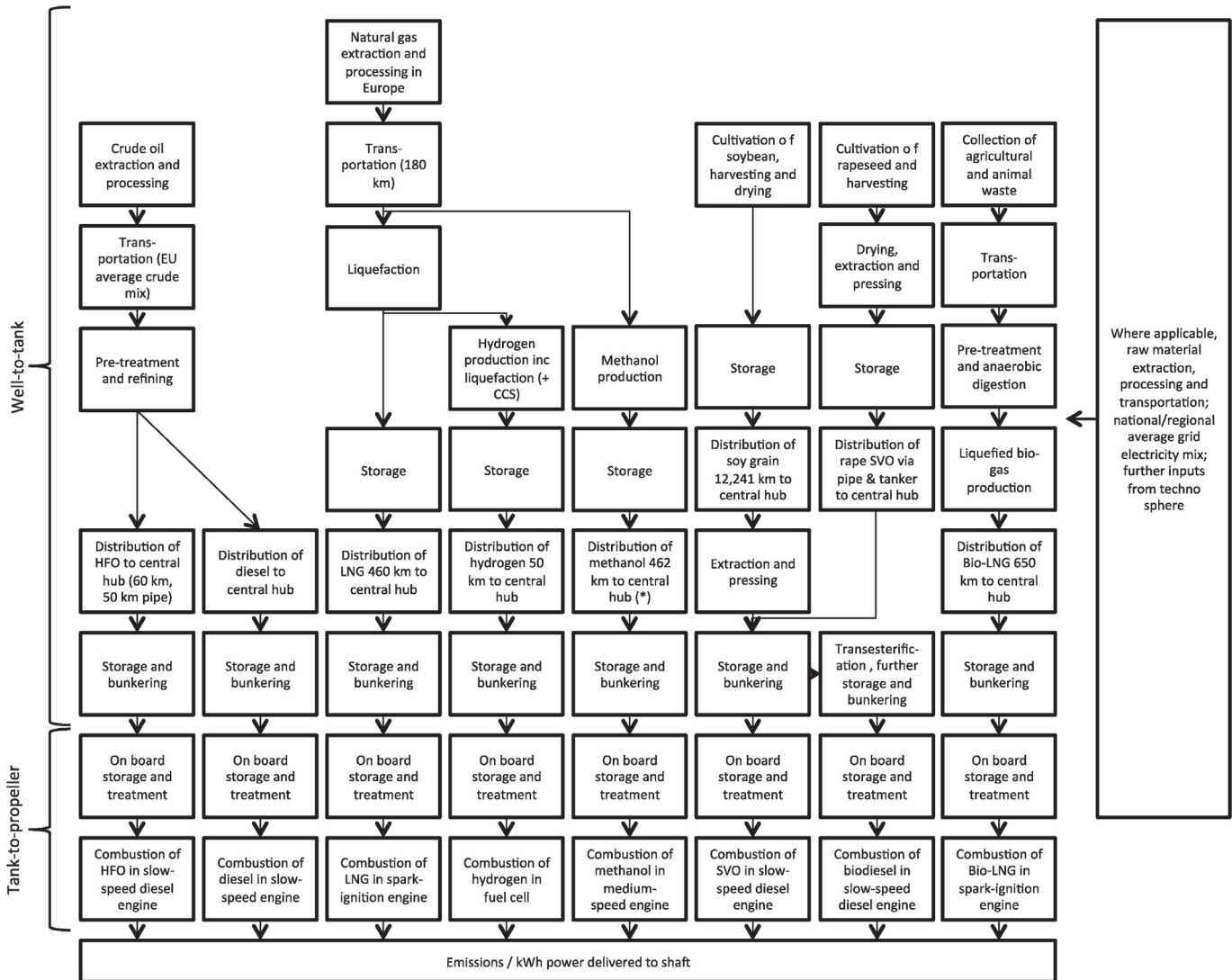
Fig. 1. Life-cycle pathways of selected alternative fuels.
