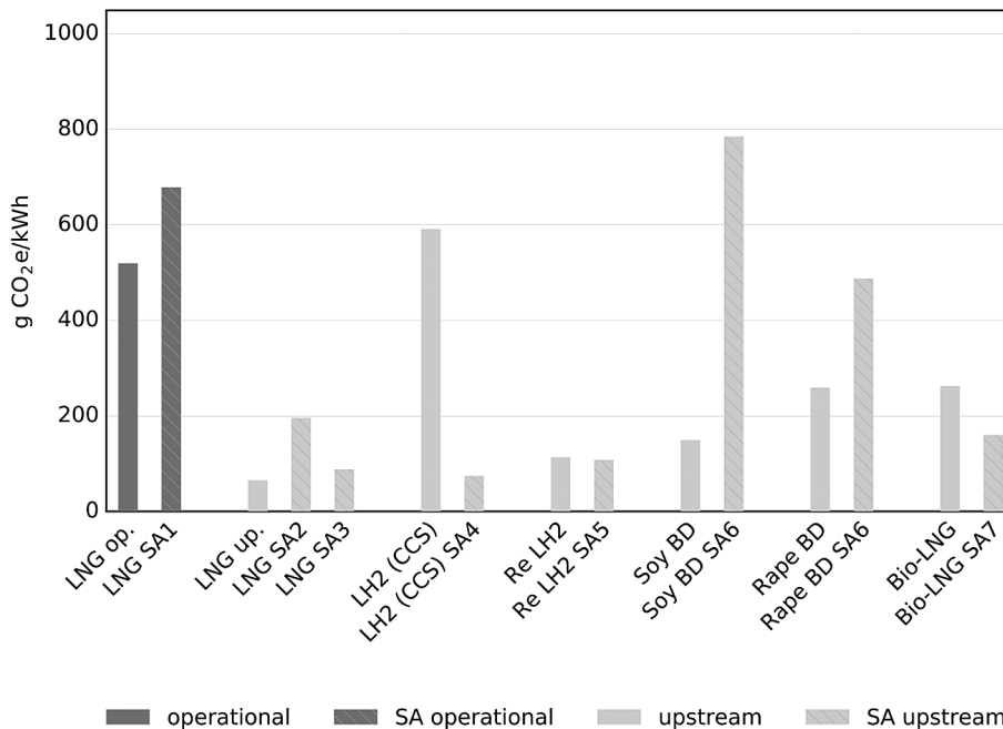
Fig. 5. Impact of sensitivity assumptions on emissions (as summarised in Table 2), measured in g CO 2 e/kWh shaft output (represented as a light grey bar), compared to baseline estimates presented in Fig. 3 (represented as a black bar). Note 'LNG op.' and 'LNG SA1' refer to operational emissions whilst the others refer to upstream emissions.
