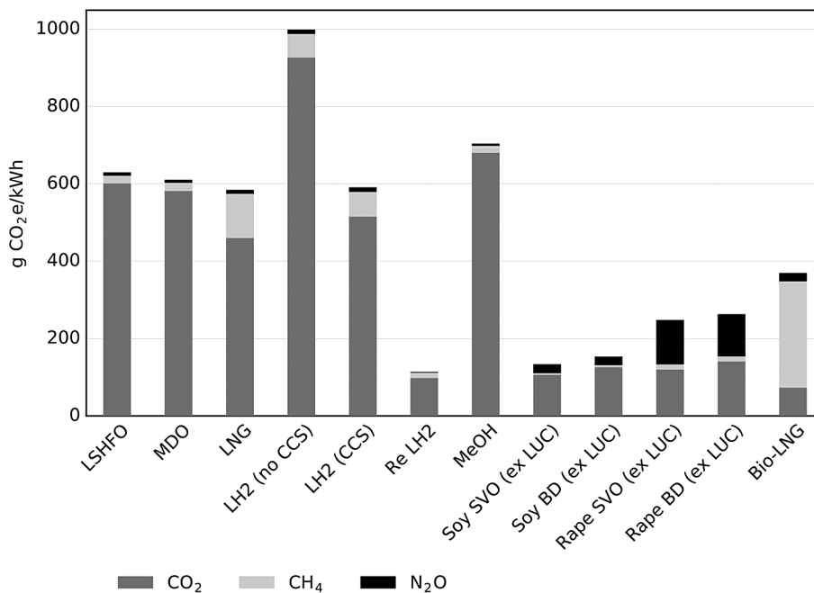
Fig. 3. Greenhouse gas emissions per kWh of shaft output, by gas species. Ex LUC denotes excluding land use change.
