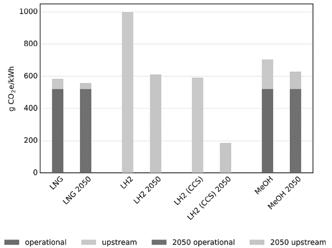
Fig. 6. Impact of temporal assumptions on life-cycle emissions summarised in Table 3, measured in g CO 2 e per kWh shaft output.
