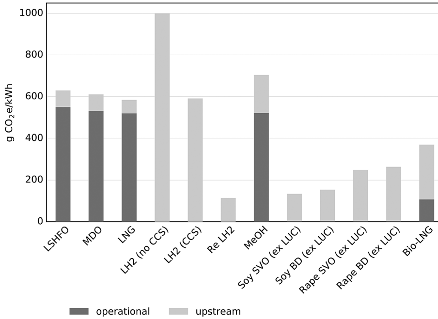
Fig. 2. Greenhouse gas emissions per kWh of shaft output, by life-cycle stage. Ex LUC denotes excluding land use change.
